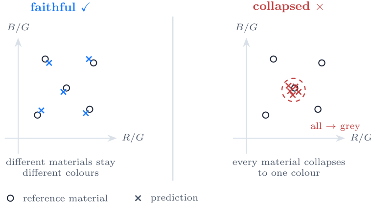
Figure 5.7: The spread ratio compares the chroma spread of the predicted materials with that of the reference. A faithful prediction keeps different materials at different colours (ratio near 1); a desaturated one collapses them towards grey (ratio well below 1), which would also make it look stable.
