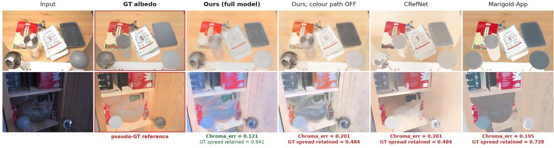
Figure 5.9: Chroma diagnostics on two distinct MIDIntrinsics test scenes and illuminant conditions (one row each). From left: the input, pseudo-GT albedo (red border), and four predictions. Albedo is defined only up to a global scale, so every panel is independently scale-normalised for display; no colour correction is applied, so the differences in saturation are differences in the predictions themselves. Values below each column are measured over the full 30-scene test split: \text{Chroma}_{\text{err}} is the pseudo-GT calibration guard and the aggregate spread ratio diagnoses collapse. The colour-path-off row and CRefNet both retain 48.4% of pseudo-GT chroma spread and have error 0.201. The “Ours” column of this figure was rendered with a later checkpoint trained for 20k further steps with additional regularisers (printed values 0.121 and 94.1%); the reported model retains 99.9% with error 0.129. The figure will be regenerated with the reported model.
