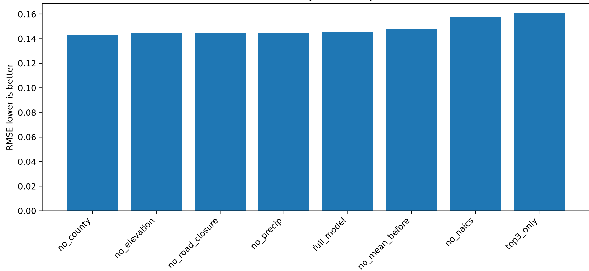
XGBoost Ablation Analysis RMSE by Feature Set
