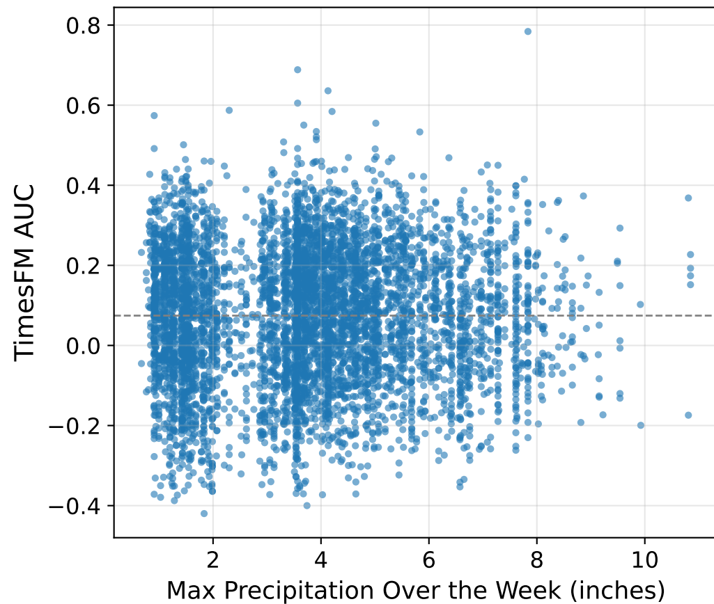
Pearson r = 0.02
