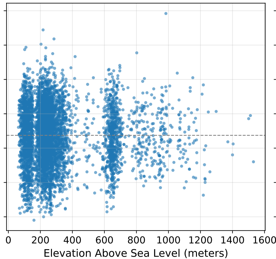
Pearson r = -0.02
