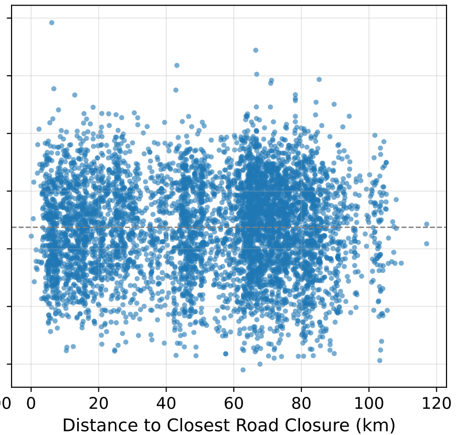
Pearson r = 0.01
