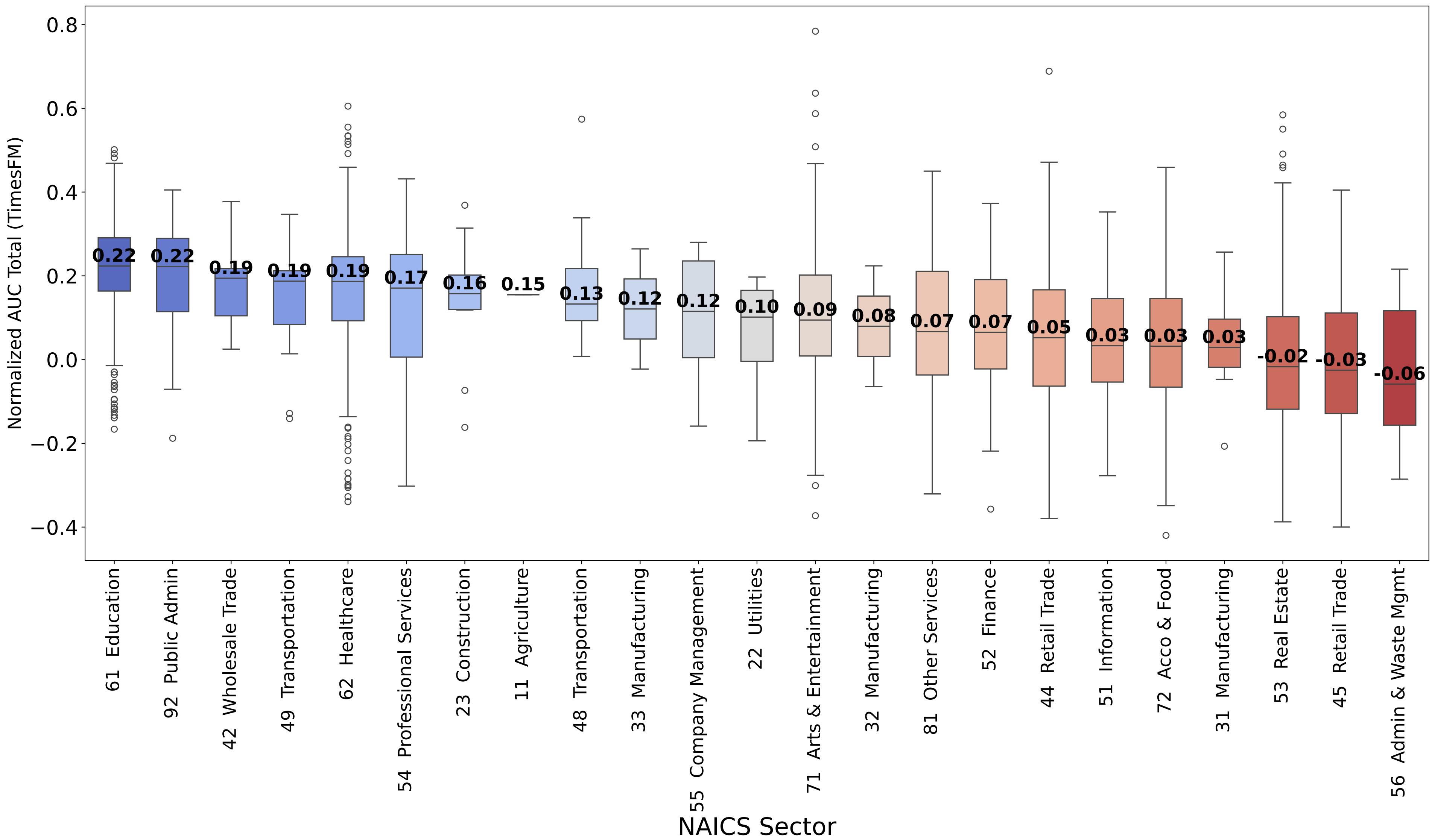
TimesFM - Normalized AUC Total by NAICS Sector
