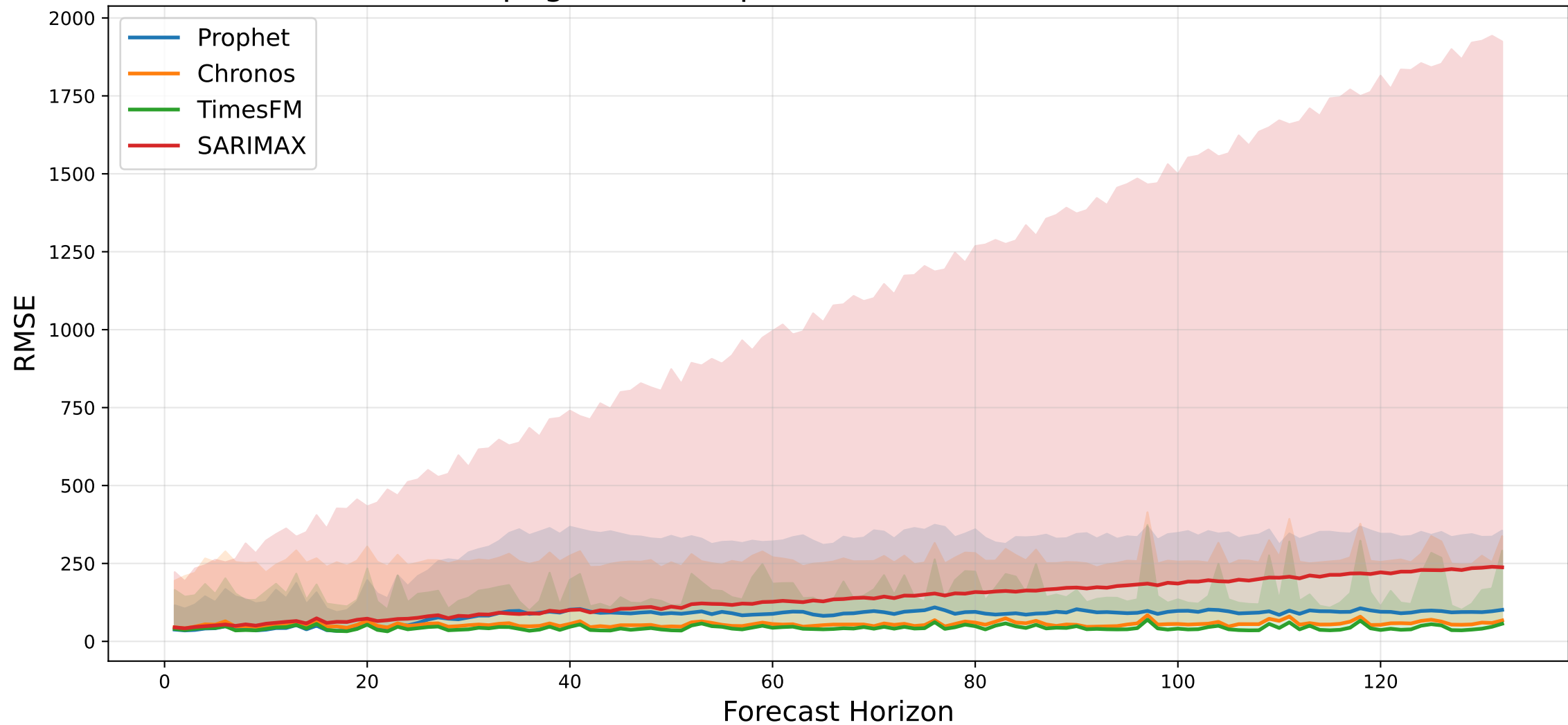
RMSE Error Propagation – Prophet vs Chronos vs TimesFM vs SARIMAX
