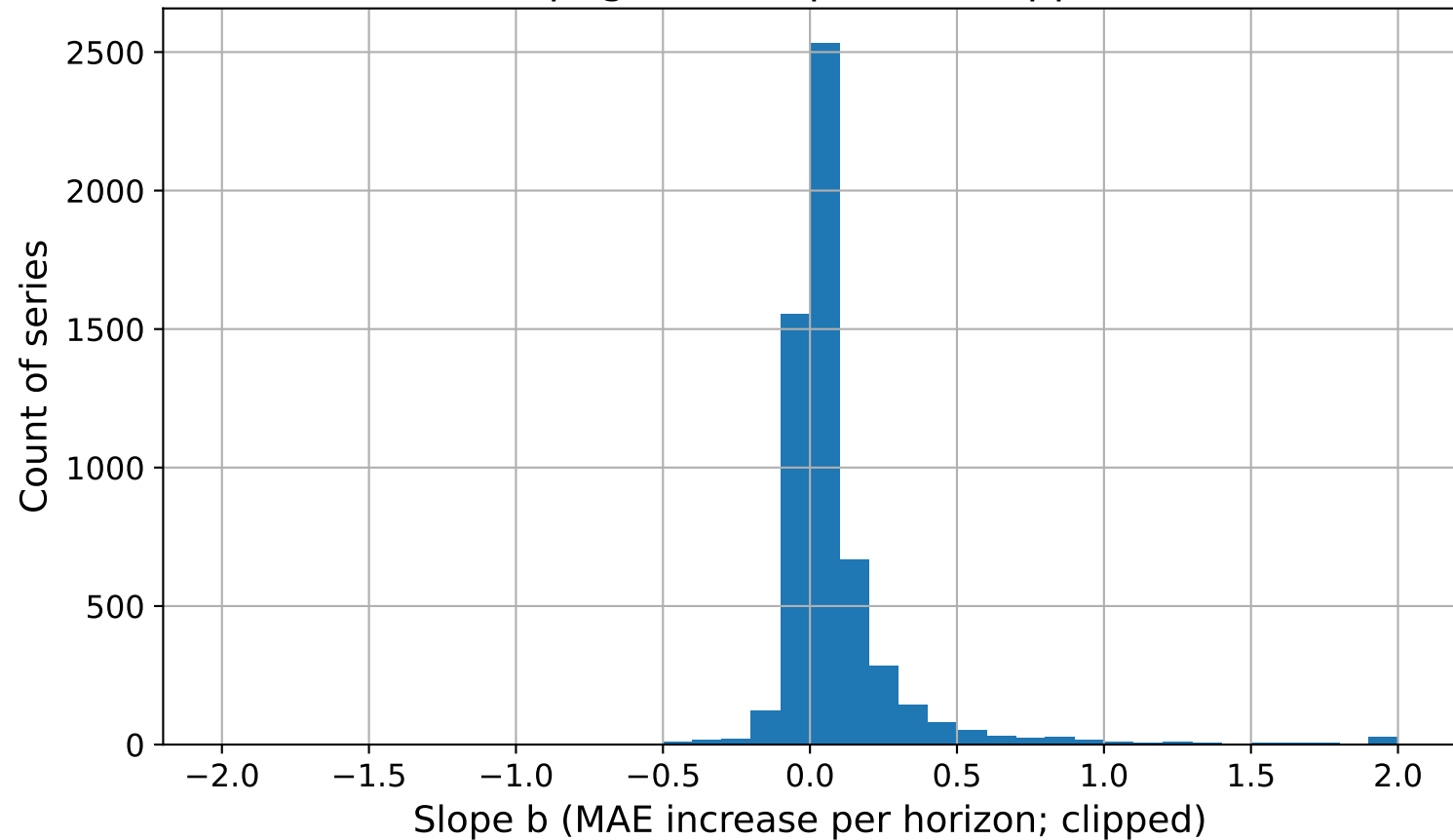
Distribution of Error Propagation Slopes (b), clipped to [-2, 2] (SARIMAX)
