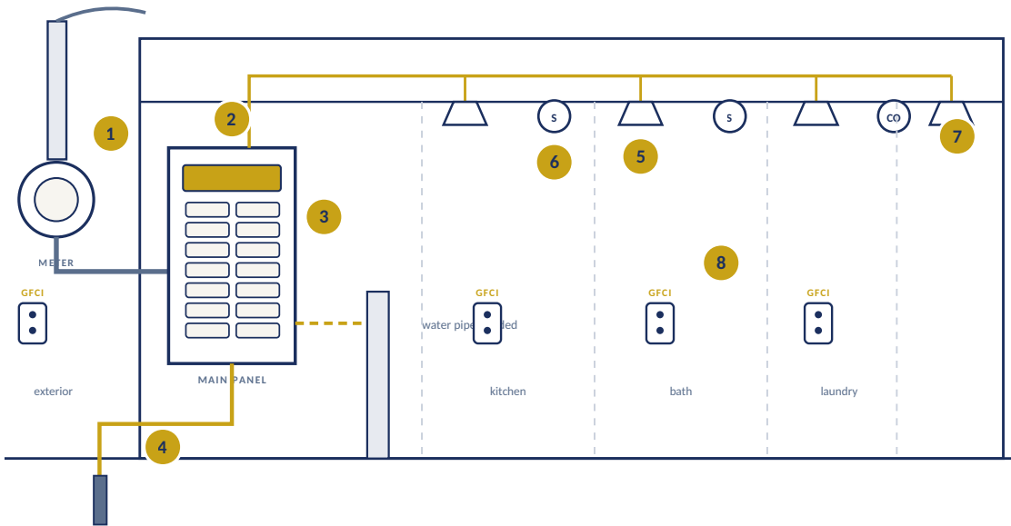
FIGURE 6 — ELECTRICAL — SERVICE, GROUNDING AND DEVICE COVERAGE
