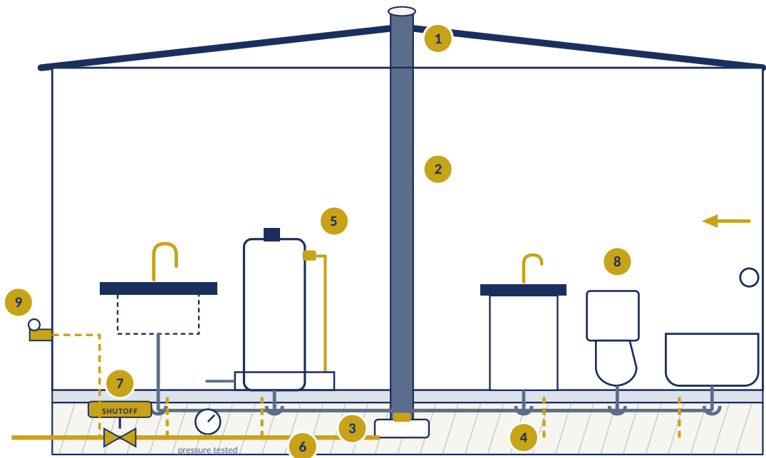
FIGURE 5 — PLUMBING — SUPPLY, DRAIN, WASTE AND VENT
