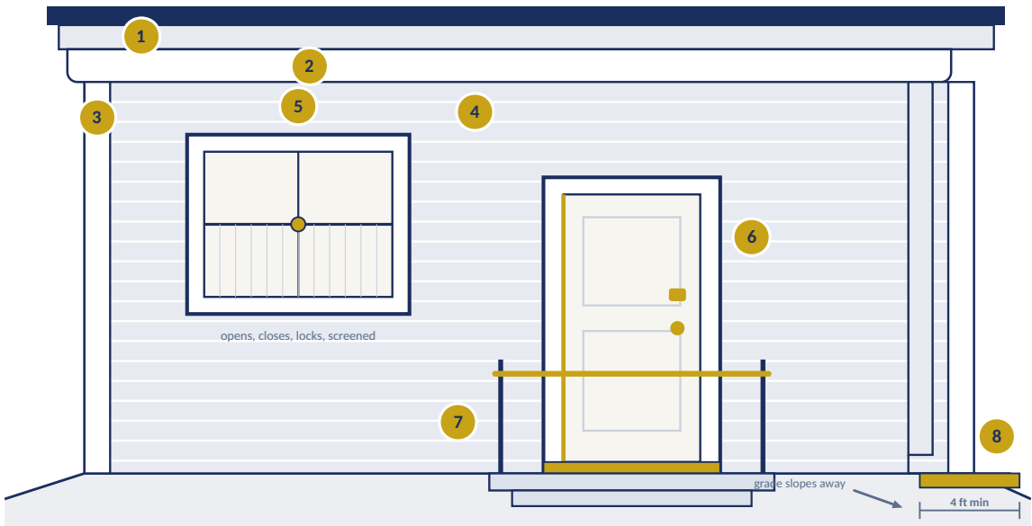
FIGURE 3 — EXTERIOR ENVELOPE — HOW THE HOUSE SHEDS WATER
