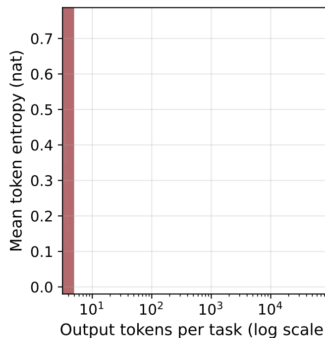
ZeroClaw
