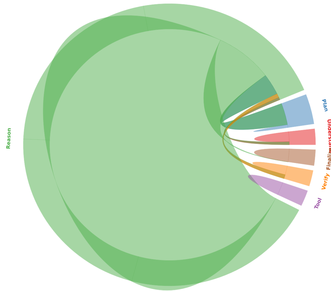
OpenClaw / success (1338)
