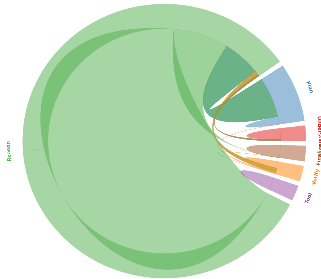
ZeroClaw / success (1442)
