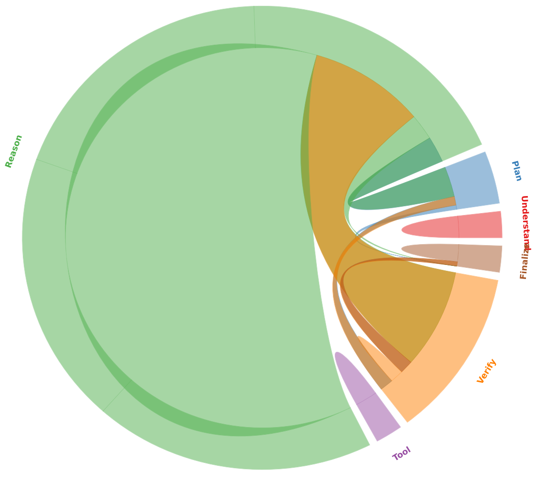
OpenClaw / failure (46)
