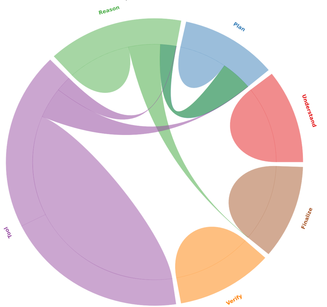
OpenClaw / failure (46)
