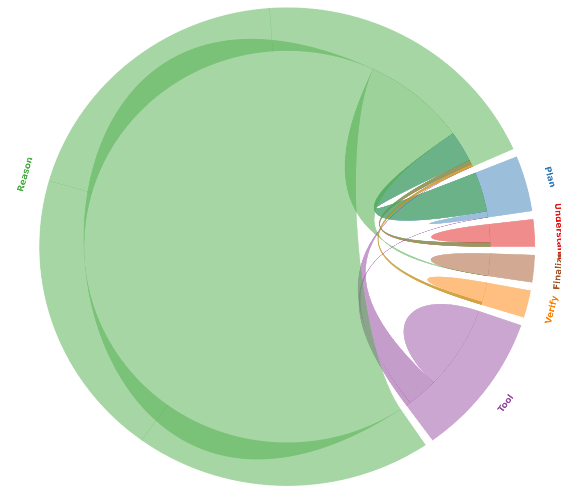
OpenCode / success (2094)
