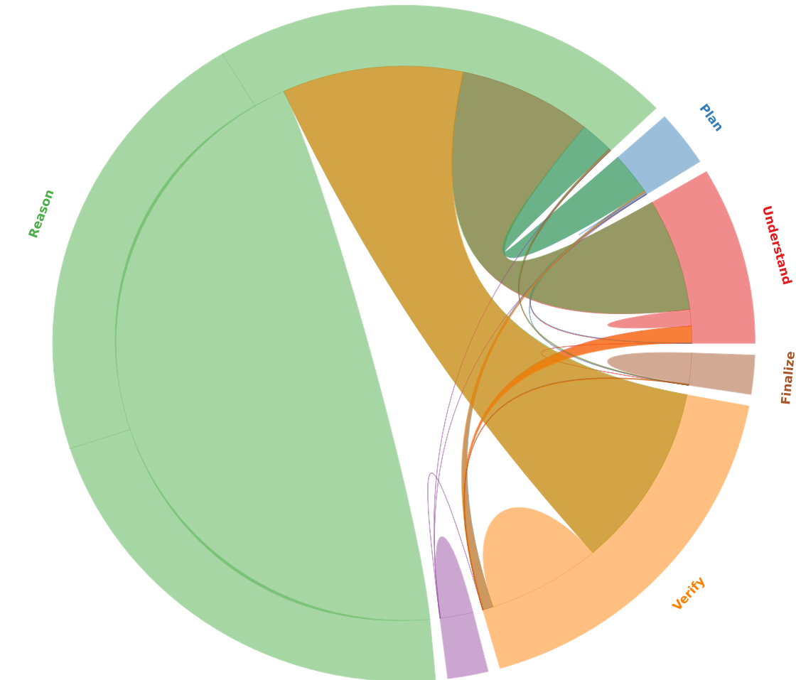
OpenCode / failure (3454)
