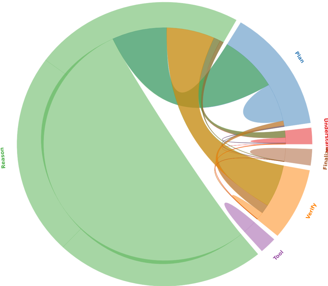
OpenClaw / success (3371)
