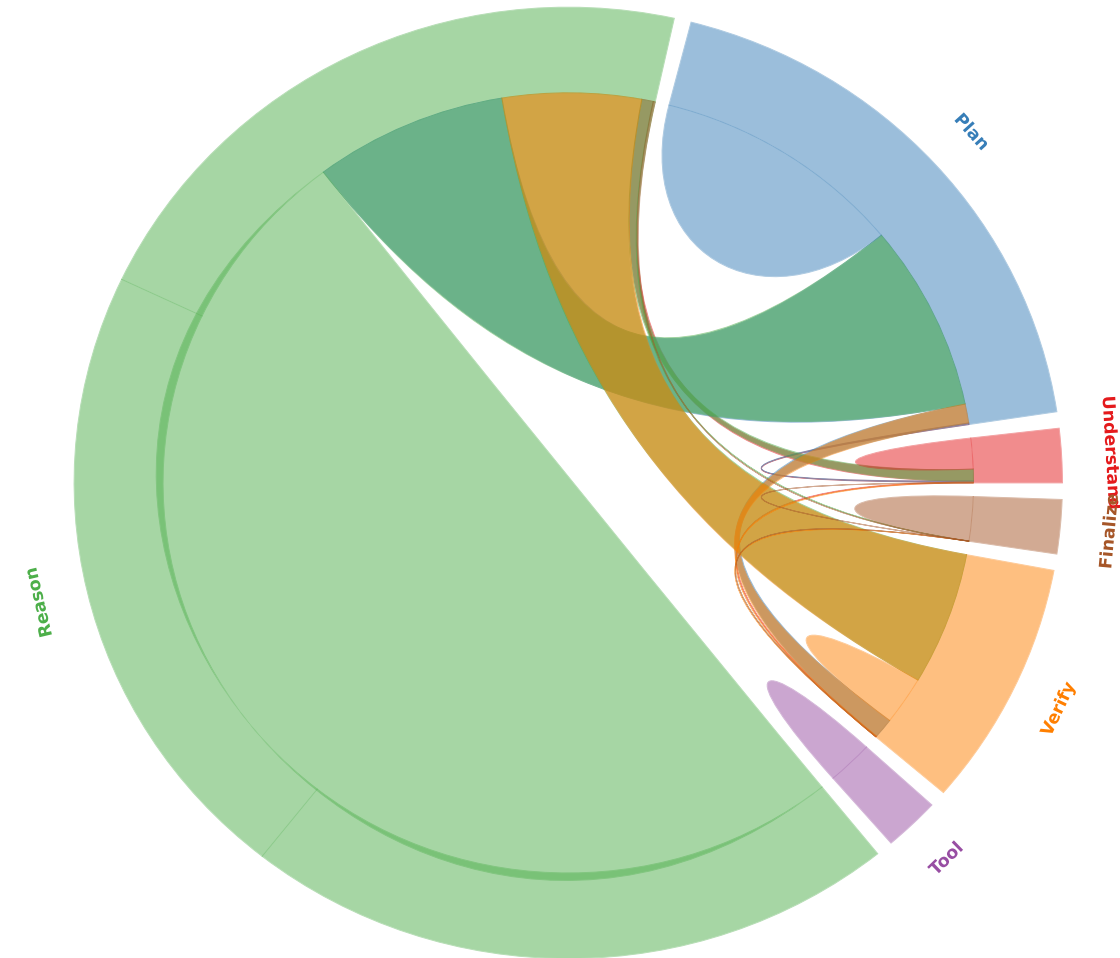
OpenClaw / failure (21279)
