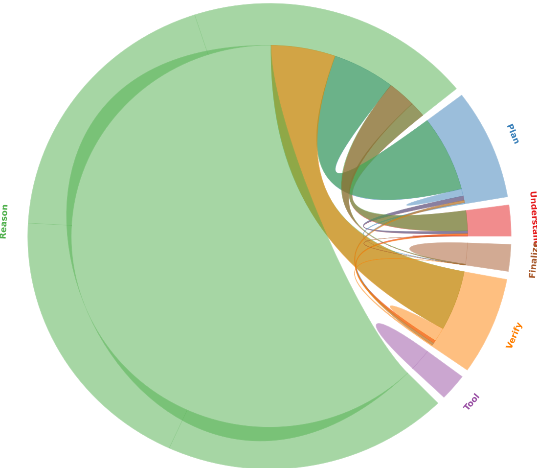
ZeroClaw / success (6150)
