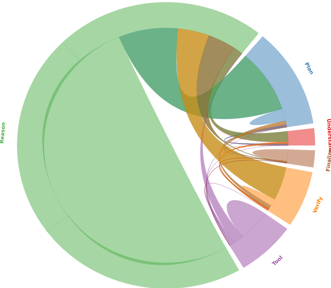
OpenCode / success (6955)
