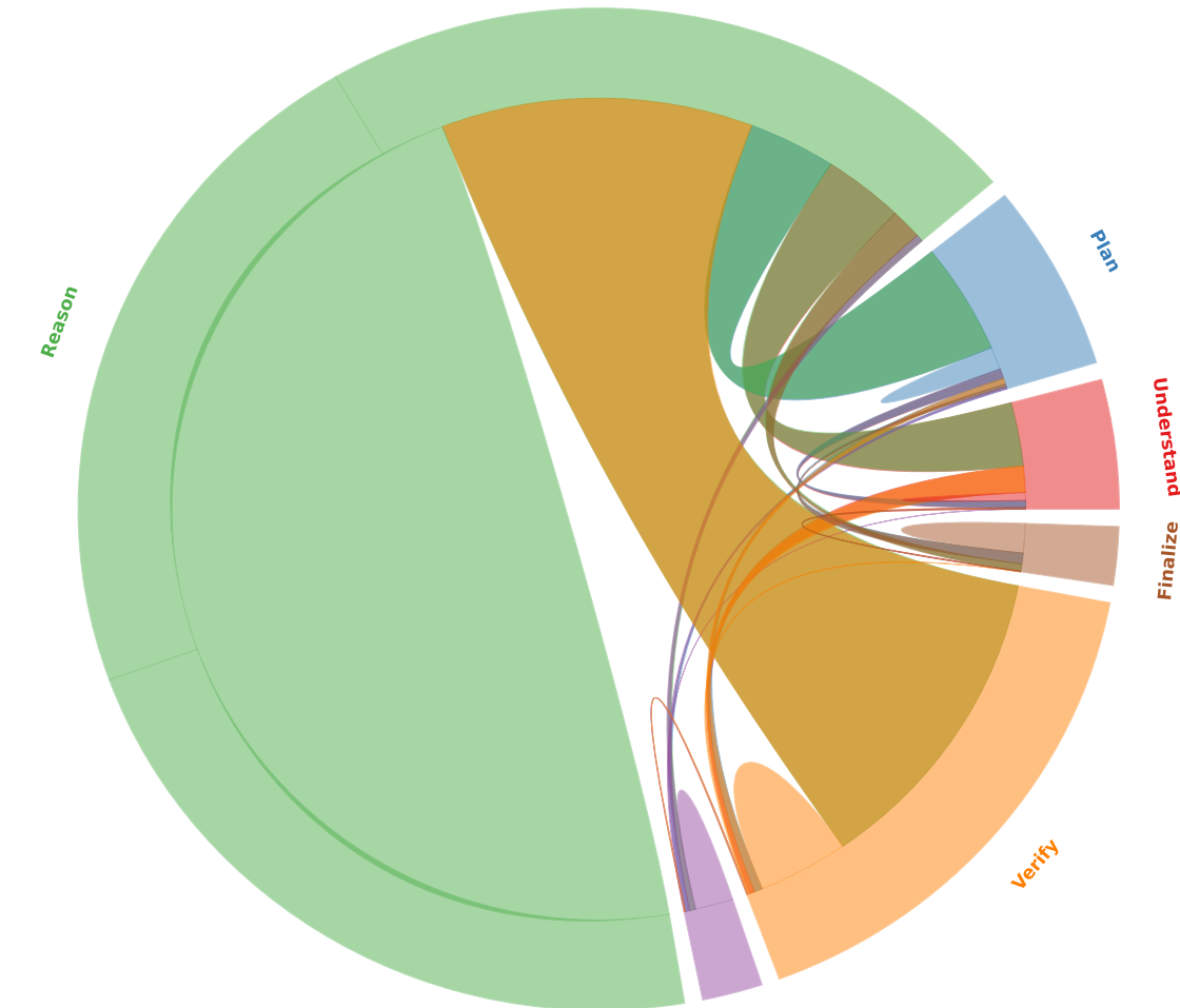
ZeroClaw / failure (1457)
