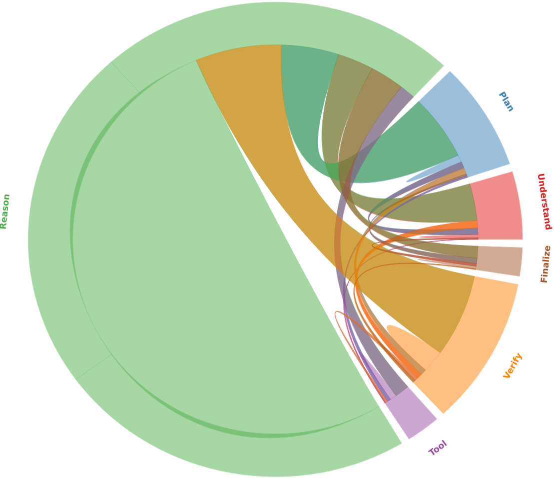
ZeroClaw / success (5002)
