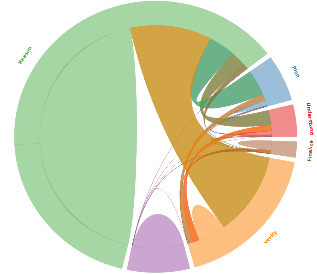
OpenCode / failure (83879)
