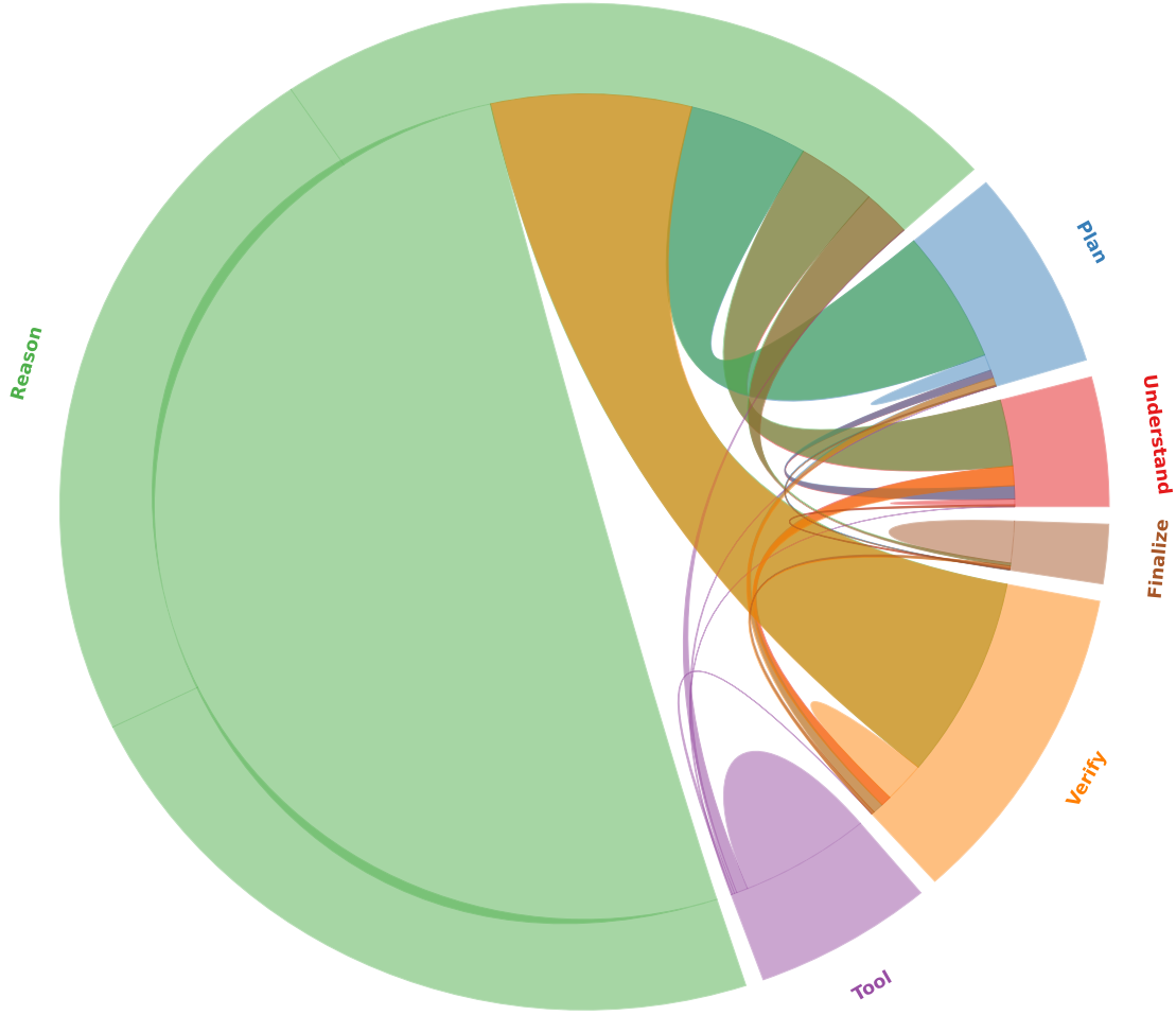
OpenCode / success (5268)
