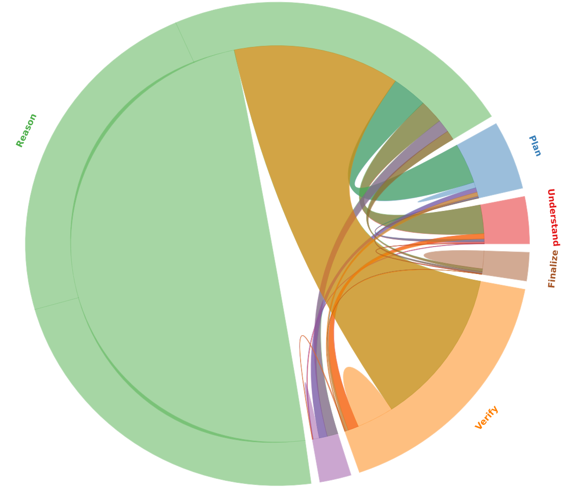
ZeroClaw / failure (21562)
