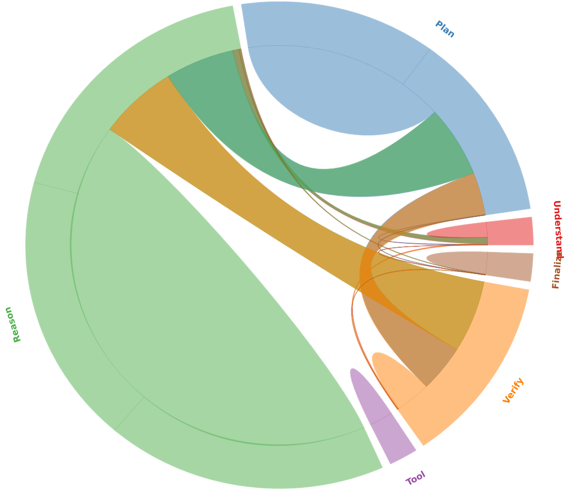
OpenClaw / failure (71534)
