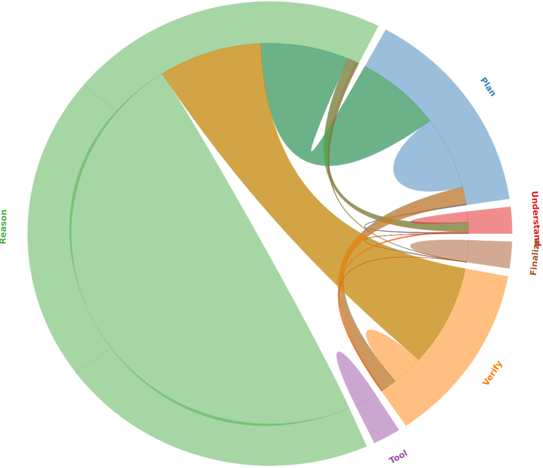
OpenClaw / success (4304)
