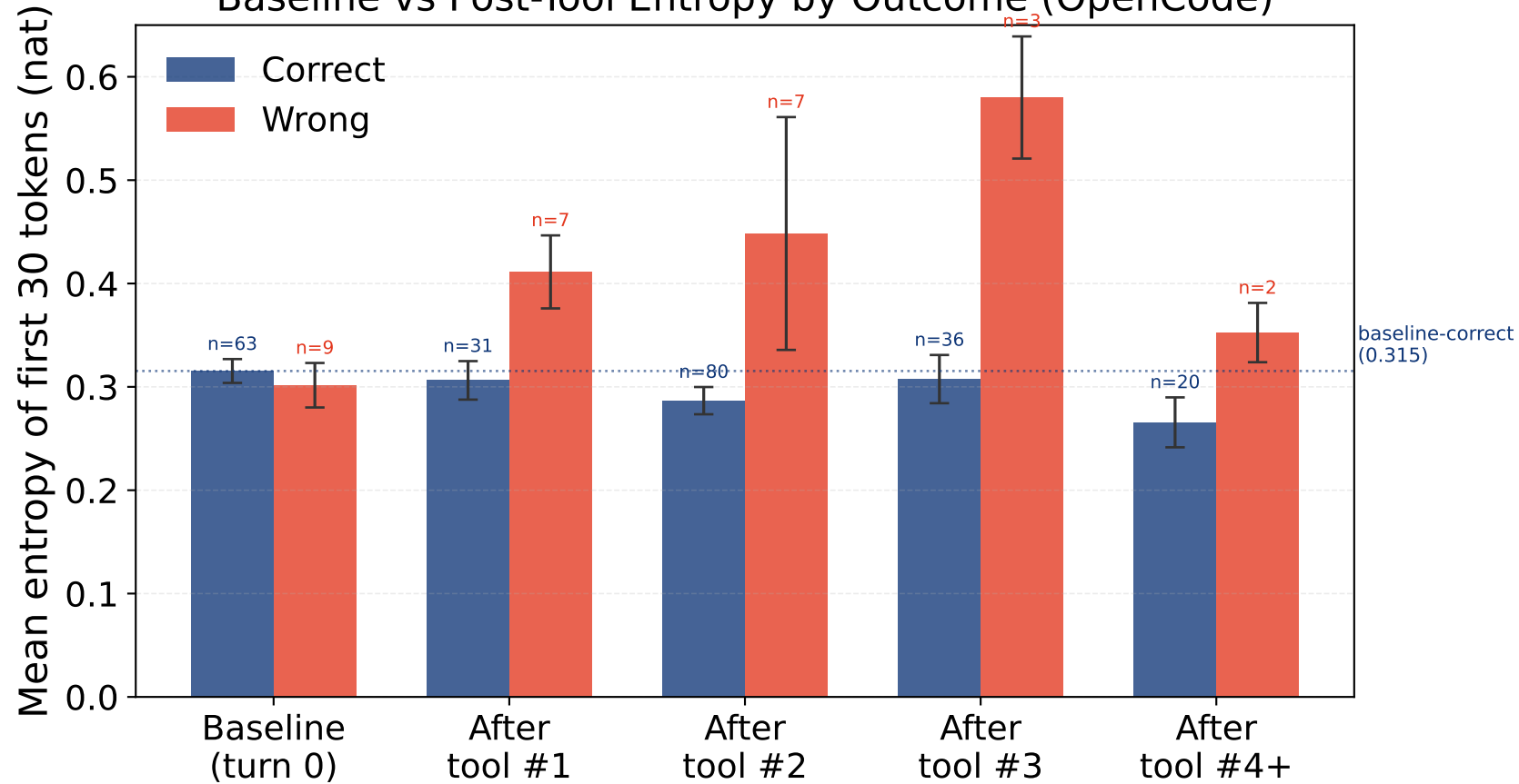
Baseline vs Post-Tool Entropy by Outcome (OpenCode)
