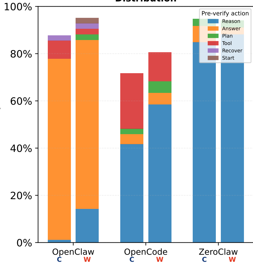
A: Pre-Verify Action Distribution
