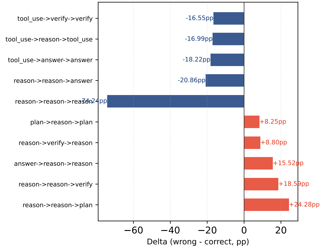
C: Motif Outcome Differences
