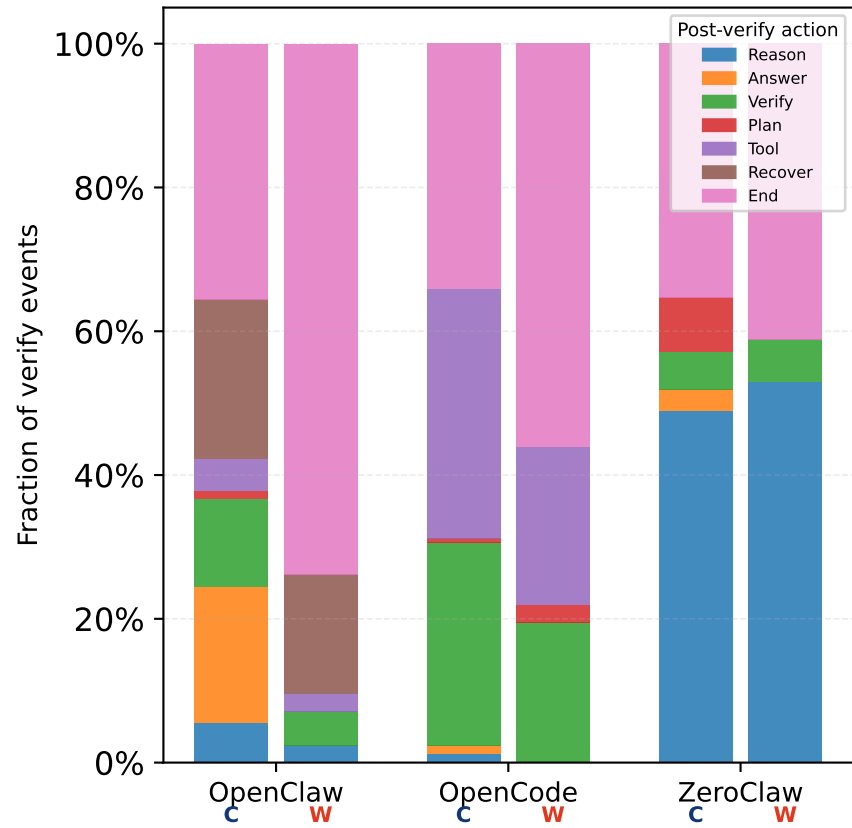
B: Post-Verify Action Distribution
