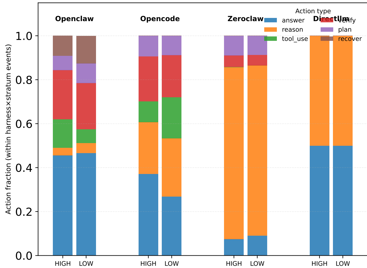
Entropy-Stratified Action Composition
