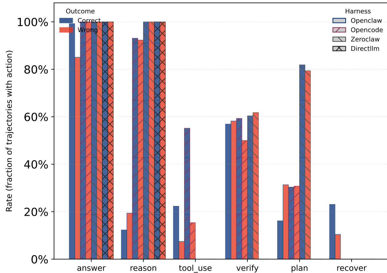
Action Rates by Harness × Outcome
