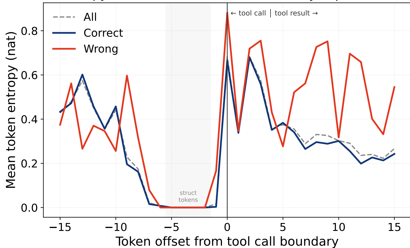
Entropy Profile around Tool Call Boundary (OpenCode)
