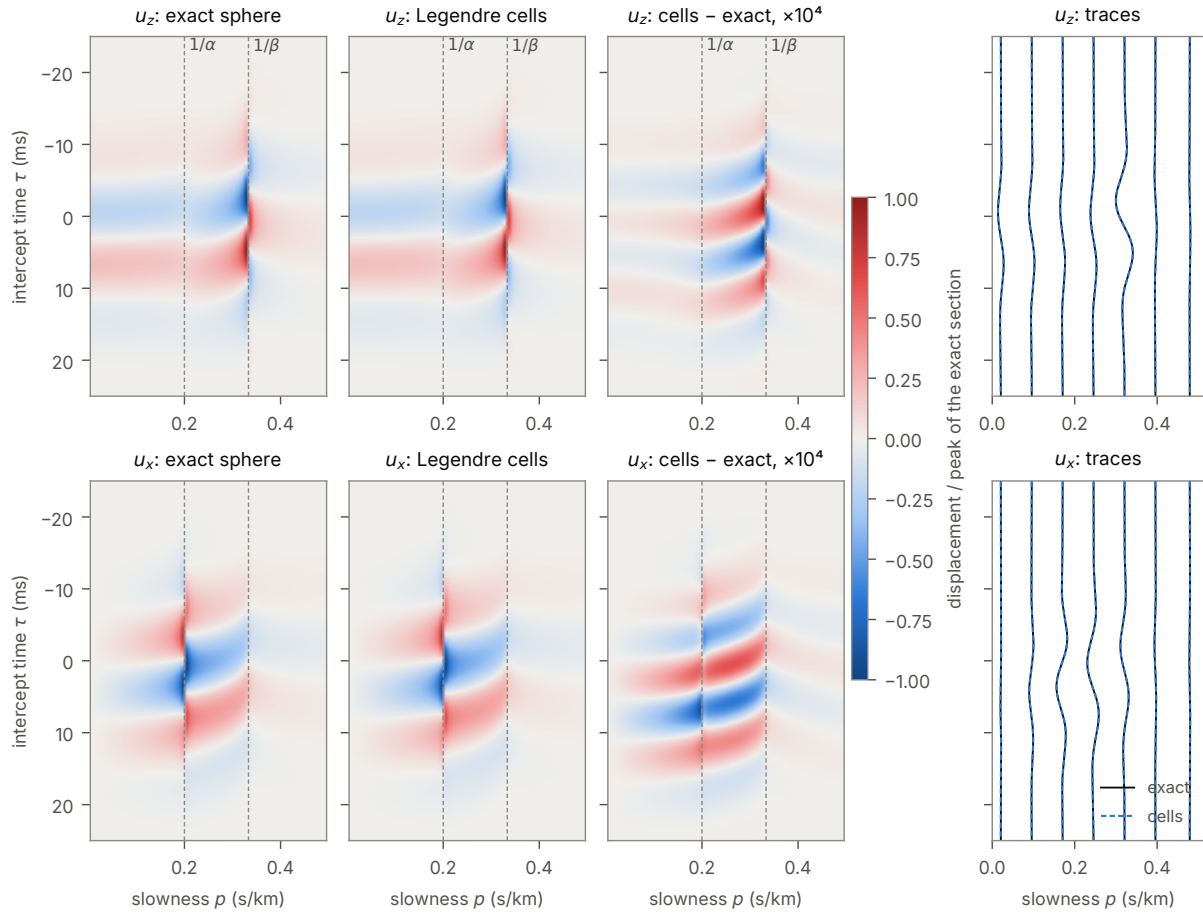
Figure 4. The \tau - p section of the graded sphere, plane P wave incident from above, receivers on a plane 1.5a above the centre: vertical ( u_z , top) and horizontal ( u_x , bottom) displacement. From the left: the exact sphere, the cell model of 8 Legendre cells of degree one across, their difference magnified 10^4 times, and traces at seven slownesses (exact solid, cells dashed). One colour scale per row, the displacement divided by the peak of the exact section; the dashed lines are the branch points p = 1/\alpha and 1/\beta . Time is measured from the passage of the incident wave through the centre of the sphere; the wavelet has zero phase and the shell above the centre scatters early, so \tau takes both signs.
