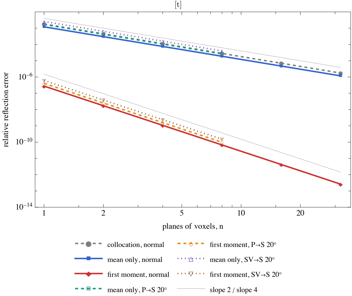
Figure 1. Relative reflection error of the discrete layer against the number of voxel planes n ( D = 2 m, \omega = 300 rad s ^{-1} , the contrast of §7). Filled: normal incidence, P reflection — collocation (§6), the mean-only voxel and the first-moment voxel of Eq. (28). Dashed, open squares and diamonds: P incident at 20°, the converted S wave, mean-only (green) and first-moment (orange) voxels of Eq. (30). Dotted, open triangles: SV incident at 20°, the reflected S wave, mean-only (purple) and first-moment (brown). Grey: slopes 2 and 4.
