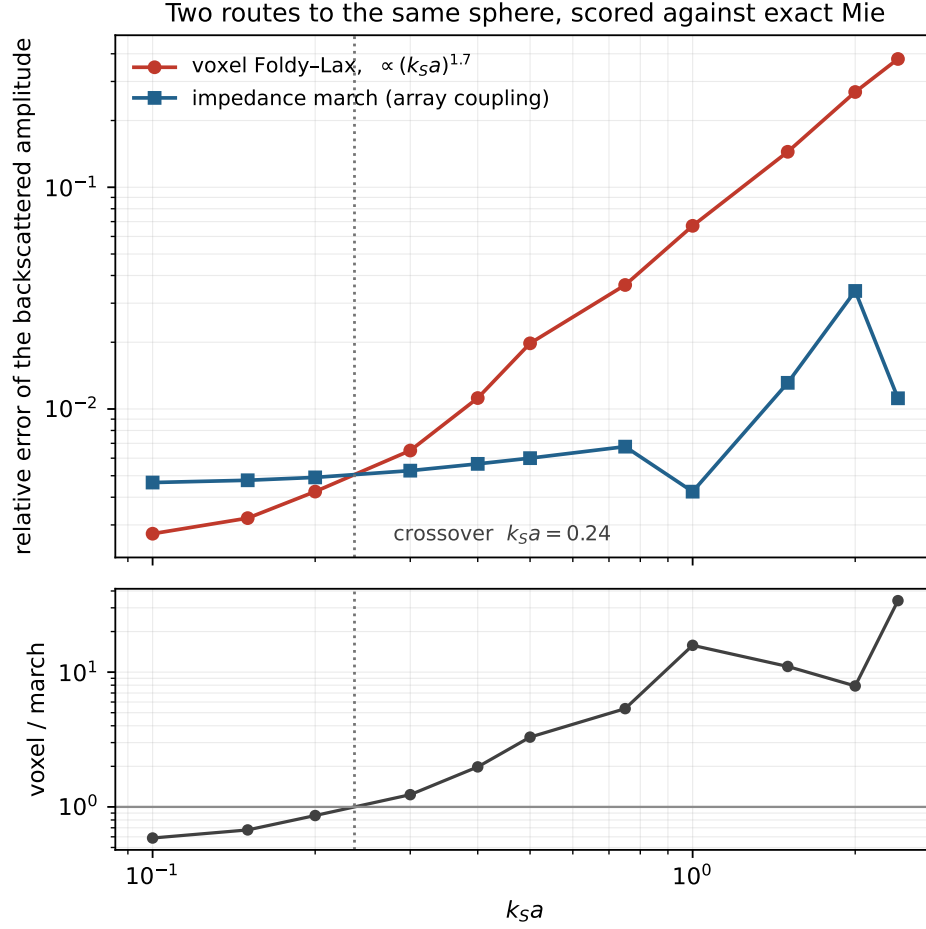
Figure 1. The same measurements. The upper panel is the error of each route against exact Mie; the lower is their ratio, crossing one at k_S a = 0.24 . The march's non-monotonicity above k_S a = 1 is the array coupling behaving as an interference rather than a decay; the voxel route's curve is a clean power law over the whole range.
