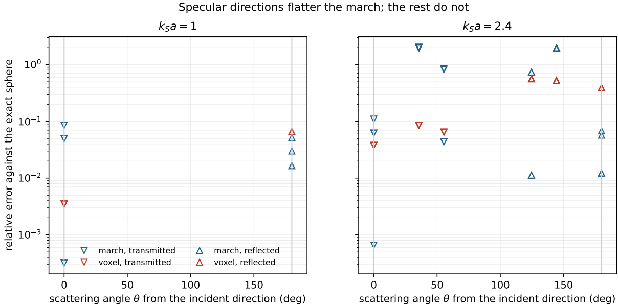
Figure 2. Every propagating order, by scattering angle. At k_s a = 1 the period supports only the specular orders; at 2.4 it supports wide-angle ones, and that is where the march’s error is of order unity.
