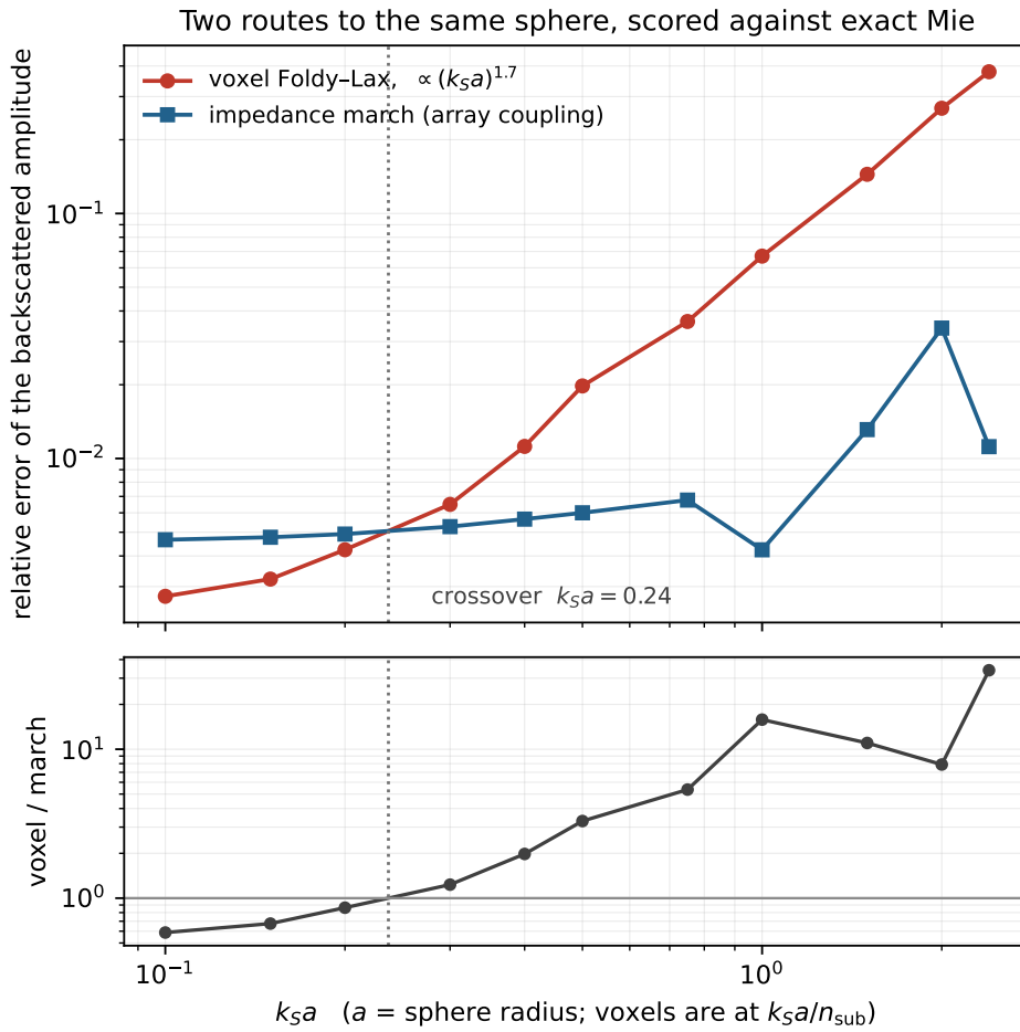
Figure 1. The same measurements. Error is |\mathbf{R}_{\text{march}} - \mathbf{R}_{\text{Mie}}|/|\mathbf{R}_{\text{Mie}}| for the march — a plane-wave coefficient (134) — and \|\mathbf{u}_{\text{FL}} - c \mathbf{u}_{\text{Mie}}\|_{\infty}/\|c \mathbf{u}_{\text{Mie}}\|_{\infty} , c = V_{\text{sphere}}/V_{\text{voxel}} , for the voxel route — a volume-corrected displacement (135). The two are not the same functional. a is the sphere ’s radius; the voxels sit at k_S a / n_{\text{sub}} , a sixth of it here. The upper panel is the error of each route; the lower is their ratio, crossing one at k_S a = 0.24 . The march’s non-monotonicity above k_S a = 1 is the array coupling behaving as an interference rather than a decay; the voxel route’s curve is a clean power law over the whole range.
