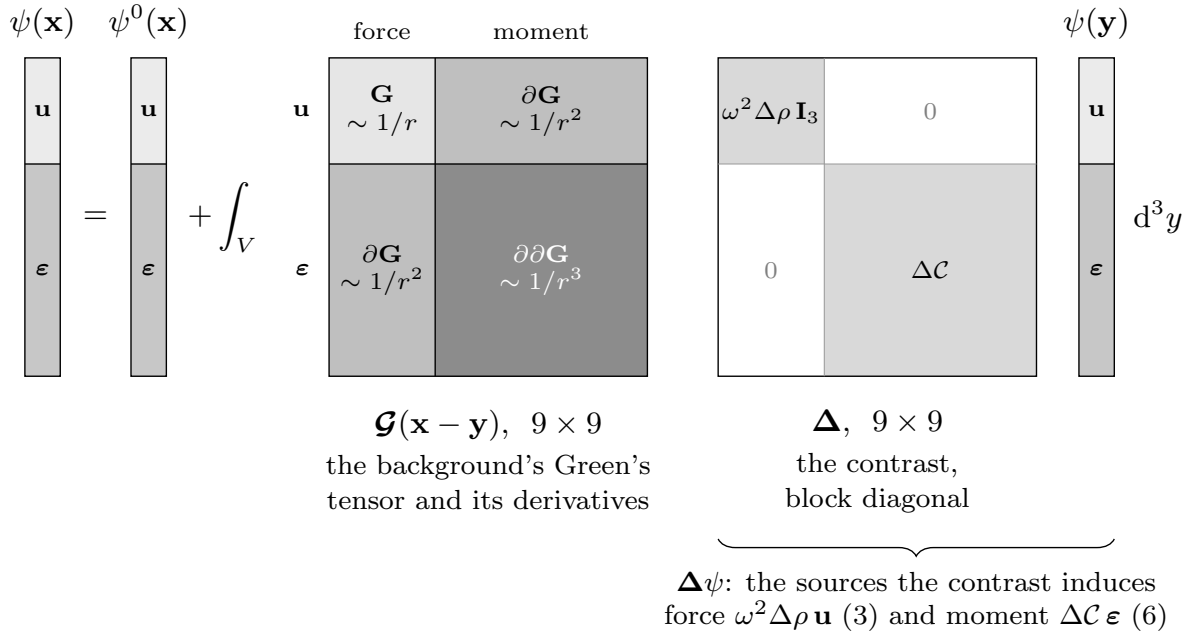
Figure 1. The nine-component Lippmann-Schwinger equation, Eq. (3), as block shapes; one unit is one component. The state \psi stacks the displacement (3) over the strain (6). The kernel's blocks carry zero, one, one and two derivatives of the Green's tensor, shaded by their singularity at \mathbf{x} = \mathbf{y} ; its columns respond to a force and to a moment, its rows give displacement and strain. The contrast \Delta is block diagonal, so the density acts only through the displacement and the stiffness only through the strain.
