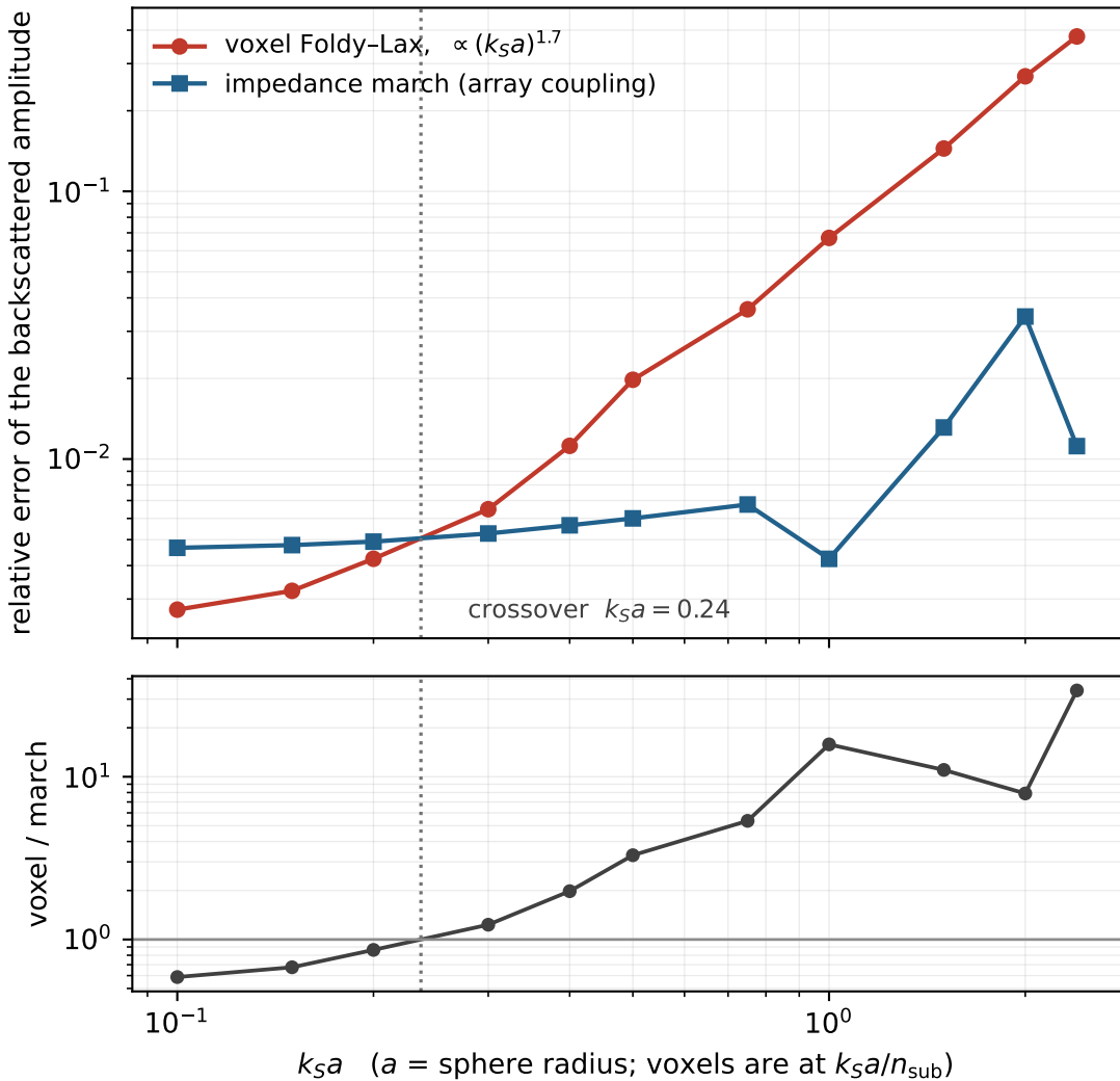
Two routes to the same sphere, scored against exact Mie
