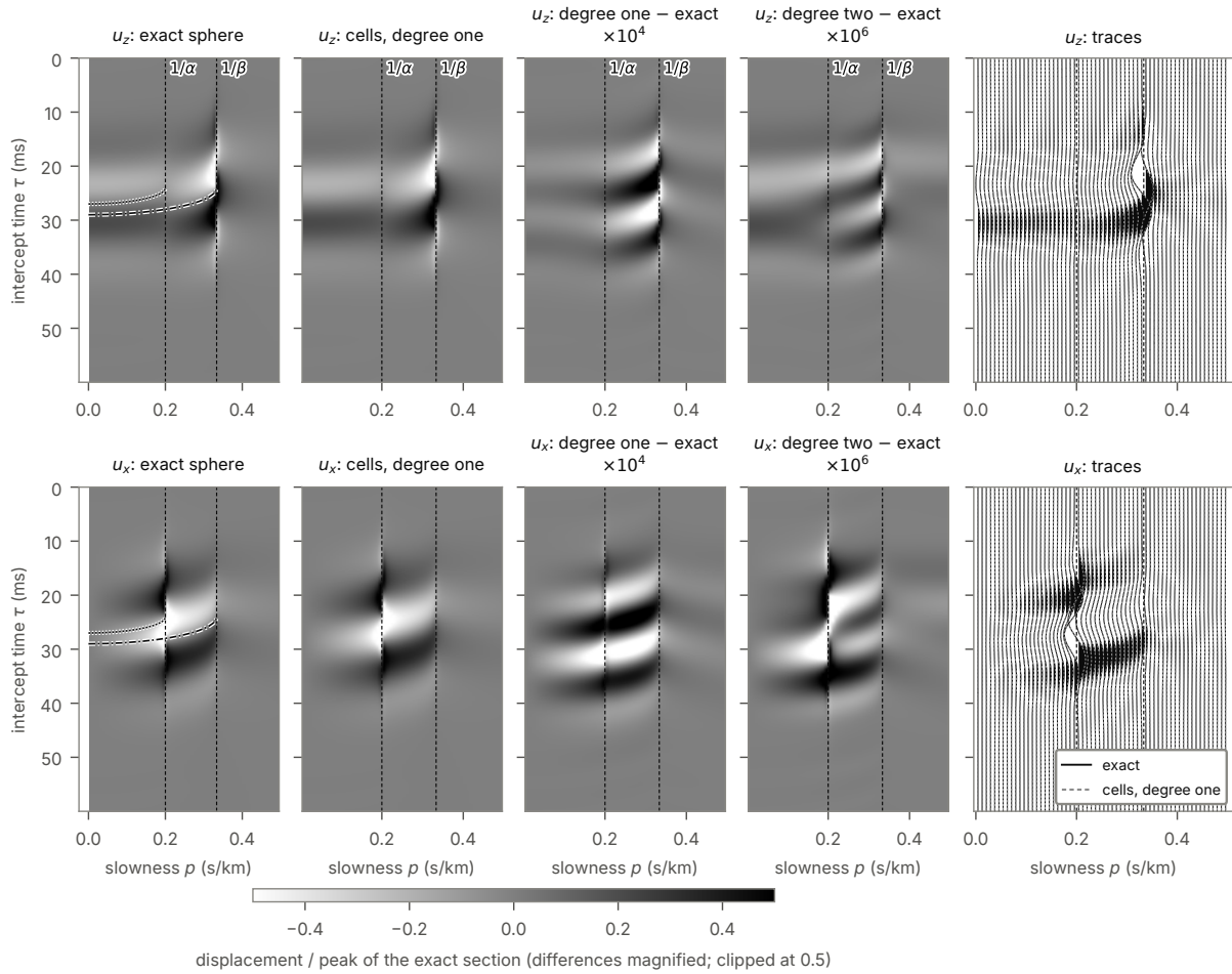
Figure 5. The \tau - p section of the graded sphere (Figure 4): plane P wave incident from above, receivers on the plane z = 0 , the centre at depth 1.5a ; vertical ( u_z , top) and horizontal ( u_x , bottom) displacement. From the left: the exact sphere; the cell model of 8 Legendre cells of degree one across; the difference of the cells of degree one and of degree two from the exact section, each magnified as marked; and the 60 traces of the section, one per slowness (exact in black with positive lobes filled, cells of degree one dashed over them). Variable density on one grey scale per row, white negative and black positive, the displacement divided by the peak of the exact section and clipped at half of it. Time runs from the incident wave's crossing of the receiver plane, with the wavelet delayed by t_d = 21 ms to be causal. The dashed verticals are the branch points p = 1/\alpha and 1/\beta ; the curves on the exact panels are the two-way times of P (dotted) and converted S (dash-dot) from the centre, t_d + z_c(1/\alpha + \eta) .
