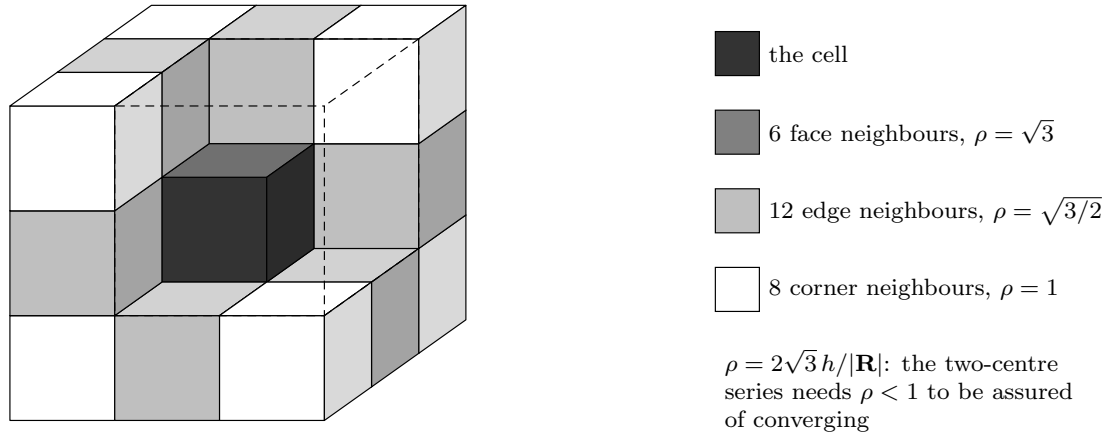
Figure 3. A cell of a space-filling tessellation and its 26 neighbours, packed face to face as in the medium. The seven neighbours in front of, above and to the right of the cell are cut away (dashed outline) so that the cell (darkest) shows. The neighbours touch it across a face (6), an edge (12) or a corner (8); for each the ratio \rho = 2\sqrt{3}h/|\mathbf{R}| of the two circumscribing radii to the distance of the centres is at least one, so none satisfies the condition under which the two-centre series is assured to converge (Table 1).
