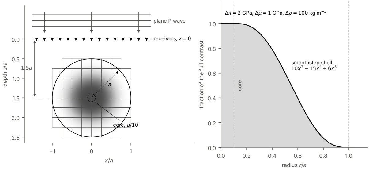
Figure 4. The graded sphere. Left: the section through the centre in the plane of incidence, shaded by the contrast, with the homogeneous core of radius a/10 (dashed), the cells of the model of 8 cells across that overlap the sphere, and the plane P wave coming down. The receiver plane and the depth axis are those of the \tau - p section of §12: receivers at z = 0 , the centre at depth 1.5a . Right: the profile, the fraction of the full contrast against the radius, 1 in the core and the smoothstep 10x^3 - 15x^4 + 6x^5 across the shell, x the fraction of the shell measured from the surface.
