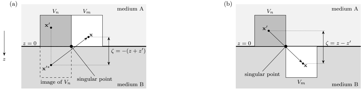
Figure 1. Cells at a welded interface, in a vertical section; z is depth. (a) Two cells in medium A that touch the interface and each other. The reflected coupling is the field of the source cell's mirror image (dashed), at the depth \zeta = -(z + z') below the field point, and the image touches the field cell at the singular point. (b) A source cell in A and a field cell in B that touch at a point of the interface. The transmitted coupling depends on \zeta = z - z' , and the singular point is where the cells touch.
