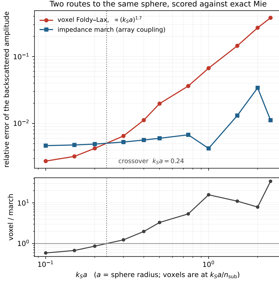
Figure 1. The same measurements. Error is |\mathbf{R}_{\text{march}} - \mathbf{R}_{\text{Mie}}|/|\mathbf{R}_{\text{Mie}}| for the march — a plane-wave coefficient (131) — and \|\mathbf{u}_{\text{FL}} - c\mathbf{u}_{\text{Mie}}\|_{\infty}/\|c\mathbf{u}_{\text{Mie}}\|_{\infty} , c = V_{\text{sphere}}/V_{\text{voxel}} , for the voxel route — a volume-corrected displacement (132). The two are not the same functional. a is the sphere ’s radius; the voxels sit at k_S a / n_{\text{sub}} , a sixth of it here. The upper panel is the error of each route; the lower is their ratio, crossing one at k_S a = 0.24 . The march’s non-monotonicity above k_S a = 1 is the array coupling behaving as an interference rather than a decay; the voxel route’s curve is a clean power law over the whole range.
