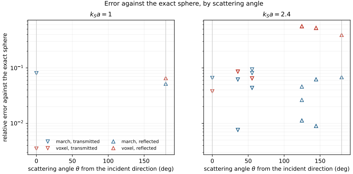
Figure 2. Every propagating order, by scattering angle, \theta measured from the incident direction so that 180^\circ is backscatter. Error is |\mathbf{R}_{\text{march}} - \mathbf{R}_{\text{Mie}}|/|\mathbf{R}_{\text{Mie}}| for the march — a plane-wave coefficient (131) — and \|\mathbf{u}_{\text{FL}} - c \mathbf{u}_{\text{Mie}}\|_{\infty}/\|c \mathbf{u}_{\text{Mie}}\|_{\infty} , c = V_{\text{sphere}}/V_{\text{voxel}} , for the voxel route — a volume-corrected displacement (132). The two are not the same functional. At k_S a = 1 the period supports only the specular orders; at 2.4 it supports wide-angle ones, and the march is the more accurate route at every one of them.
