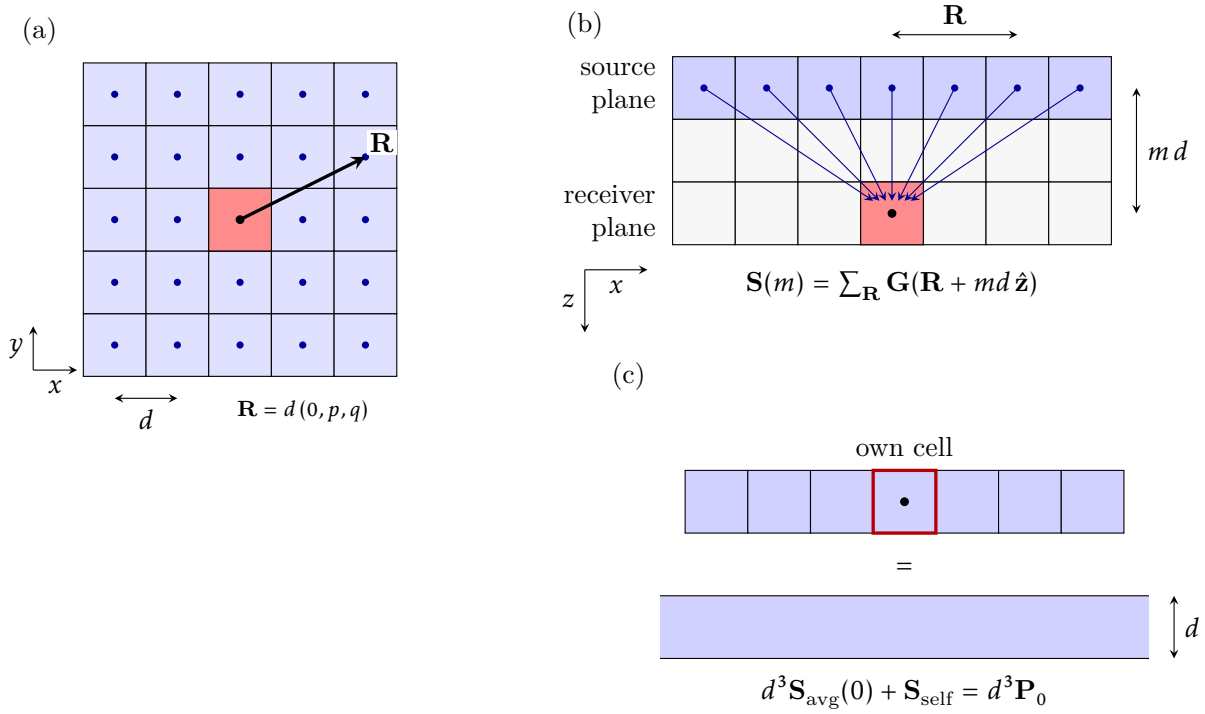
Figure 1. The lattice and its sums. (a) Plan view of one plane of voxels: their centres form a square lattice of pitch d , and a lattice vector \mathbf{R} = d(0, p, q) joins the centre of one voxel (red) to another. (b) Cross-section ( z down), between planes: the voxel of a receiver plane (red) is coupled to every voxel of a source plane m planes above it, one for each lattice vector \mathbf{R} ; the sum over \mathbf{R} is the specular lattice sum of Eq. (4). (c) Within a plane: the sum over every cell of the plane, the receiver’s own cell (outlined) included, is the field of a uniform plate of thickness d , the tiling identity of Eq. (10).
