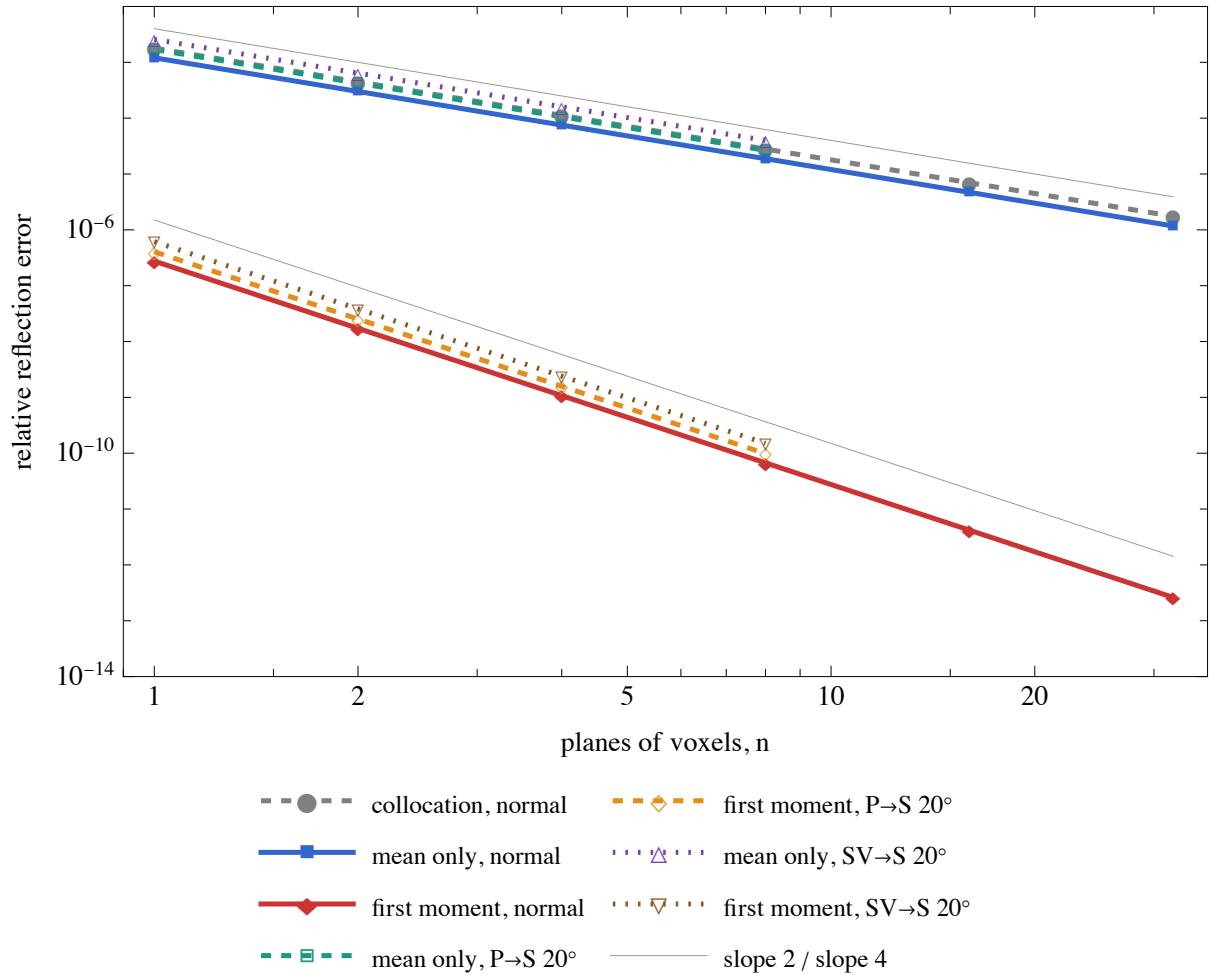
Figure 1. Relative reflection error of the discrete layer against the number of voxel planes n ( D = 2 m, \omega = 300 \text{ rad s}^{-1} , the contrast of §7). Filled: normal incidence, P reflection: collocation (§6), the mean-only voxel and the first-moment voxel of Eq. (28). Dashed, open squares and diamonds: P incident at 20^\circ , the converted S wave, mean-only (green) and first-moment (orange) voxels of Eq. (30). Dotted, open triangles: SV incident at 20^\circ , the reflected S wave, mean-only (purple) and first-moment (brown). Grey: slopes 2 and 4.
