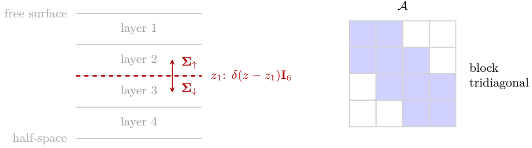
Figure 1: Left: the layer stack, with a source plane at z_1 radiating \Sigma_\uparrow upward and \Sigma_\downarrow downward. Right: the global matrix \mathcal{A} of (3). Each interface couples only neighbouring layers, so \mathcal{A} is block tridiagonal — which is what the Riccati recursion of §3 exploits.
