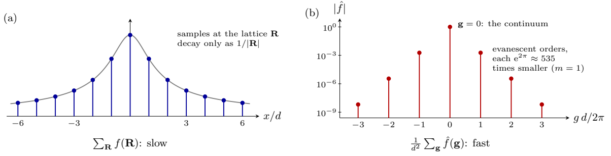
Figure 2. The Poisson summation formula (9) applied to a plane of voxels, along one lateral axis. (a) Real space: the field of each voxel of a source plane at a receiver one plane away, sampled at the lattice points; the samples decay only as 1/|\mathbf{R}| , so their sum converges slowly. (b) The same sum after Poisson summation, on a logarithmic scale: samples of the lateral Fourier transform at the reciprocal-lattice orders \mathbf{g} = 2\pi\mathbf{p}/d . The order \mathbf{g} = 0 is the continuum's plane wave; every other order is evanescent and, at m = 1 , smaller than its neighbour by e^{2\pi} \approx 535 . Magnitudes are schematic: the static decay e^{-|\mathbf{g}|md} is shown.
