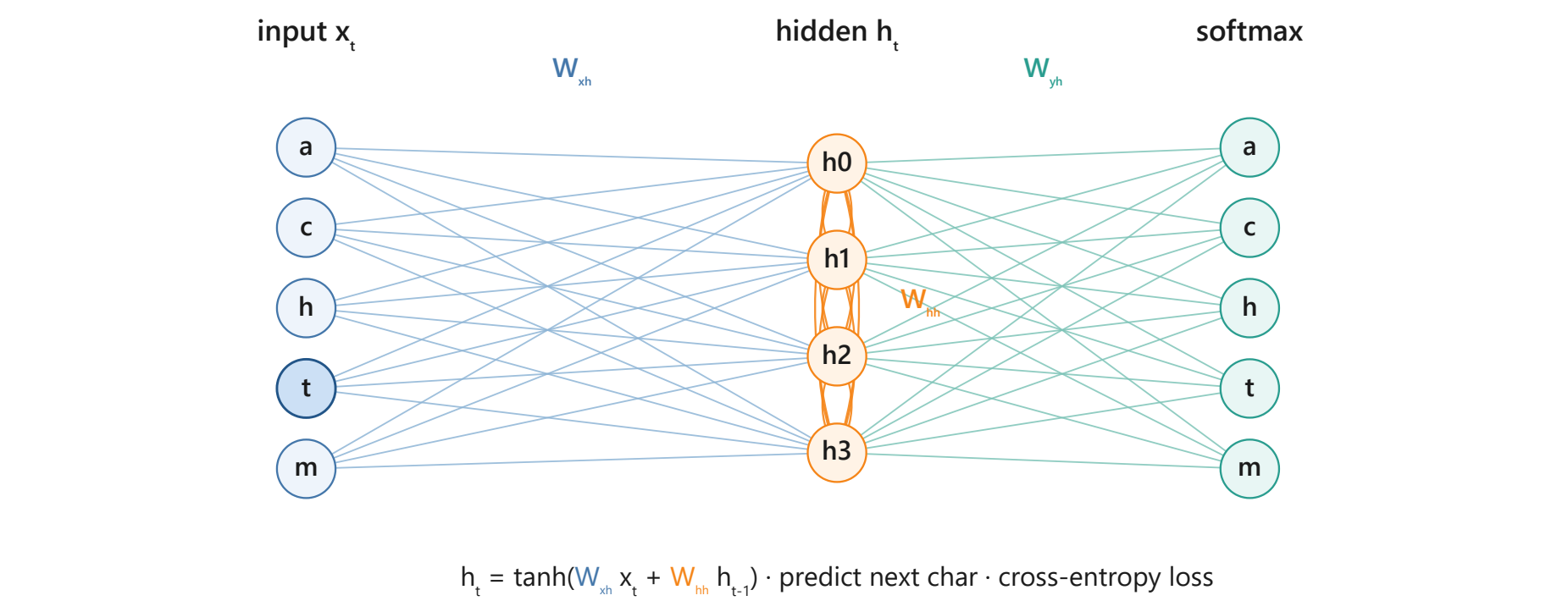
Fig 2 · Training the RNN
