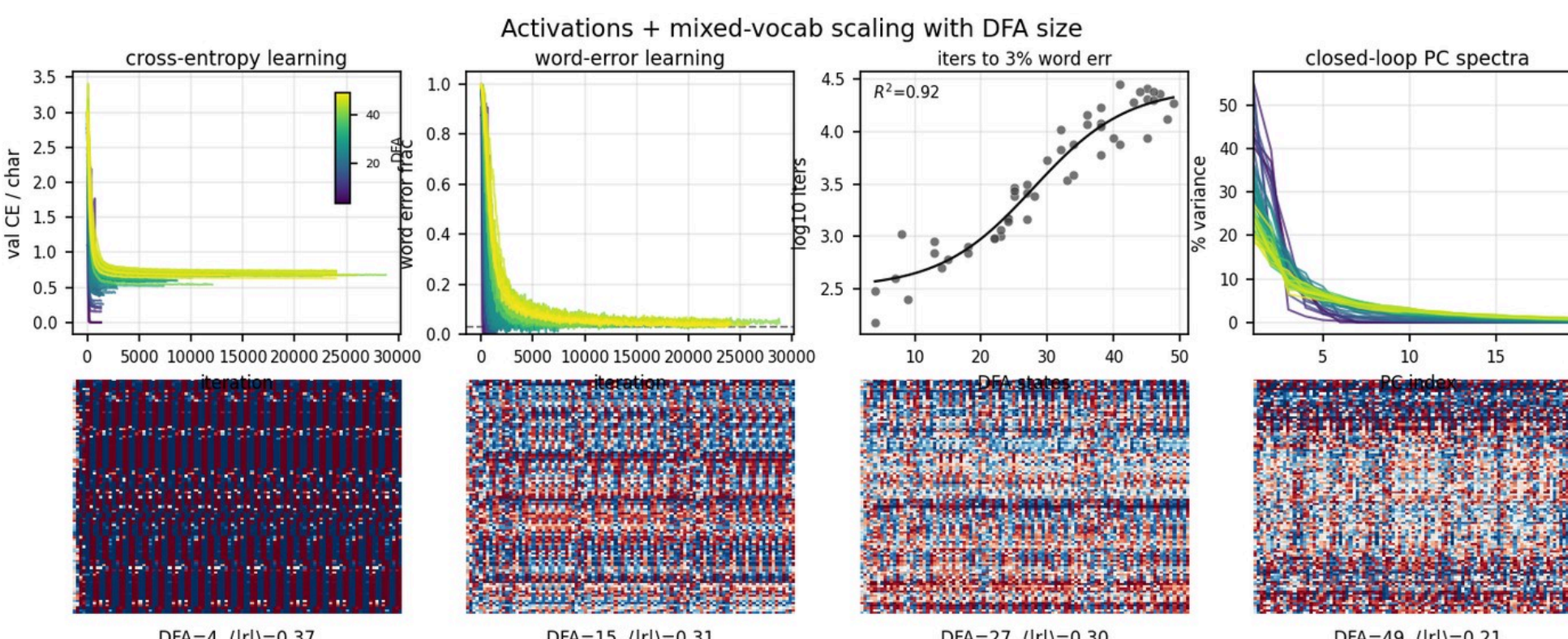
Fig 12 · Activations & scaling vs DFA size
