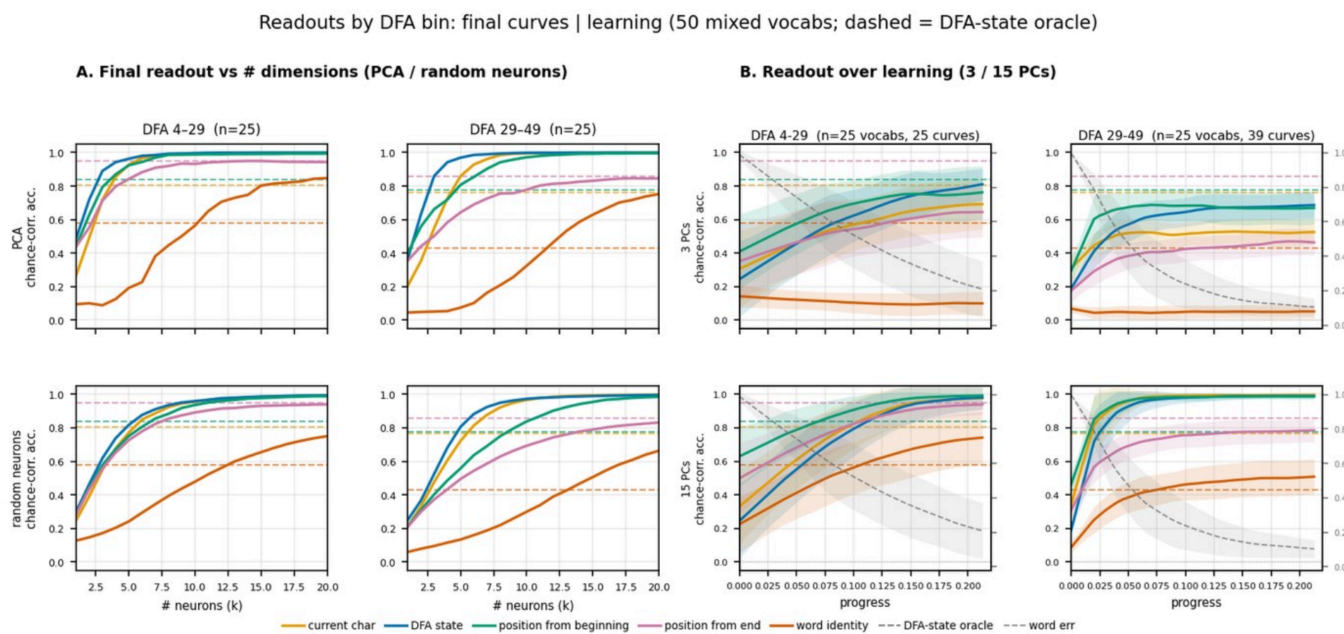
Fig 15 · Readouts vs DFA size
