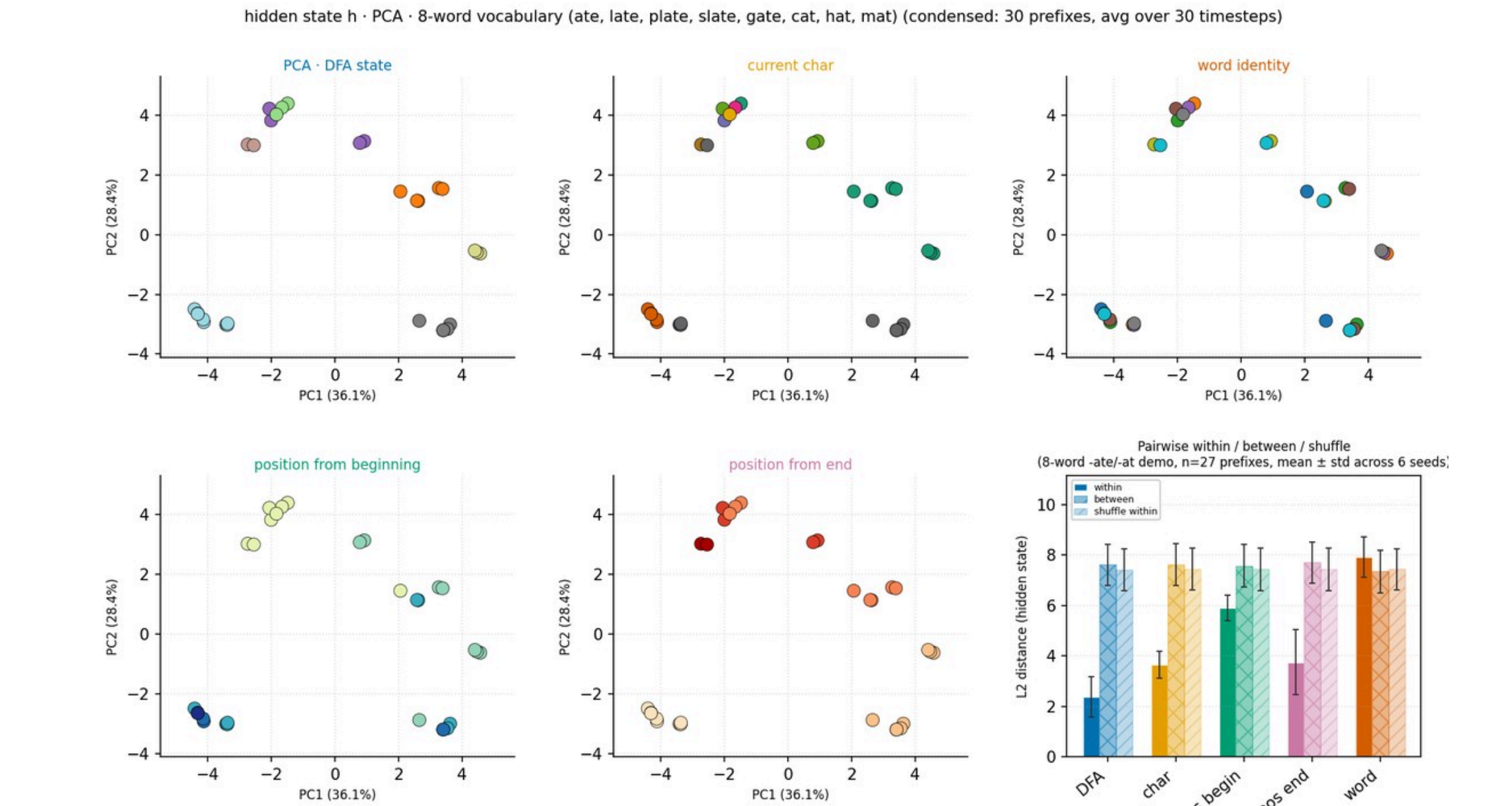
Fig 8 · DFA geometry & separation
