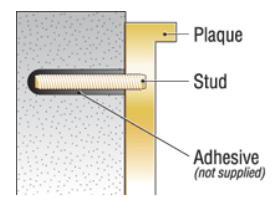
Blind Stud Mount with pattern
