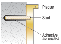
Blind stud mounting with pattern.
