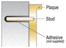
Blind Stud Mount with pattern
