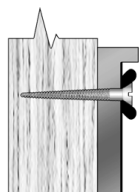
(4) Countersunk Wood Screw mount
