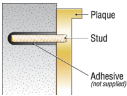
Blind Stud Mount with pattern
