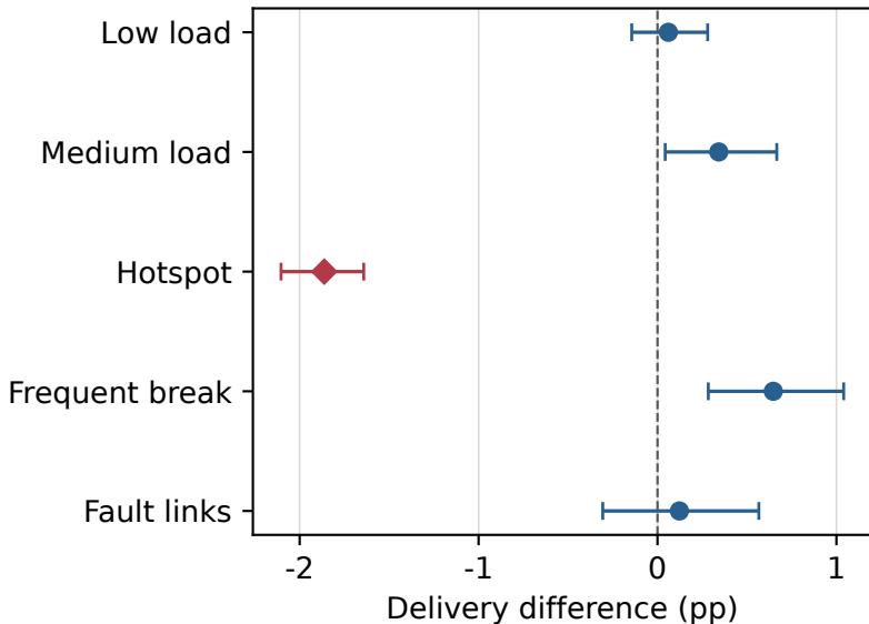
(a) Delivery (MAPPO - Q-routing)
