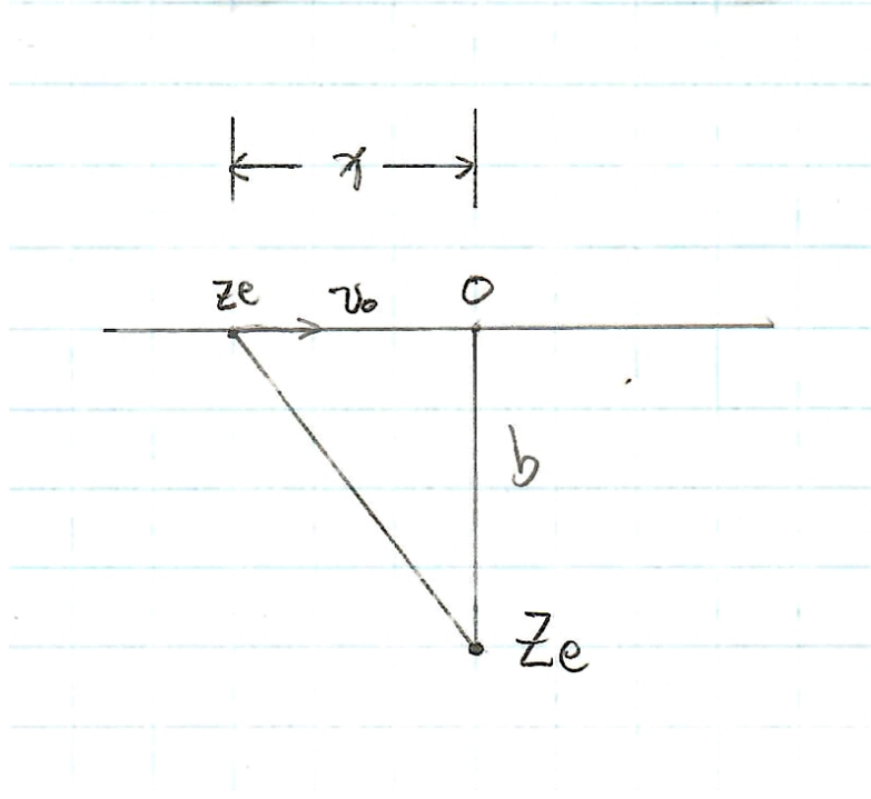
Figure 1: Non-relativistic particle moving in a straight line.
