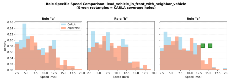
Fig. 4: Role-specific speed distribution comparison for the lead vehicle in front with neighbor vehicle scenario. Green rectangles mark identified coverage gaps where Argoverse shows sufficient density but CARLA is nearly empty. Role “a” = ego vehicle, role “b” = lead vehicle, role “c” = neighbor vehicle.
