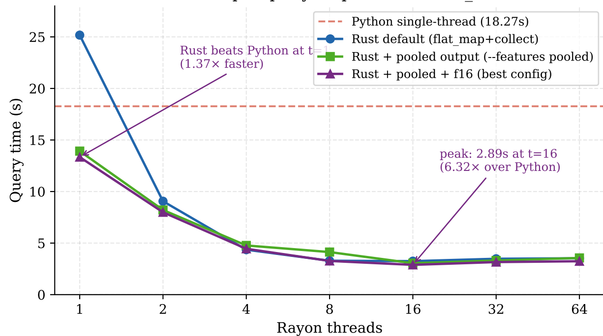
Pre-allocated per-query output Vec — eval\_medium
