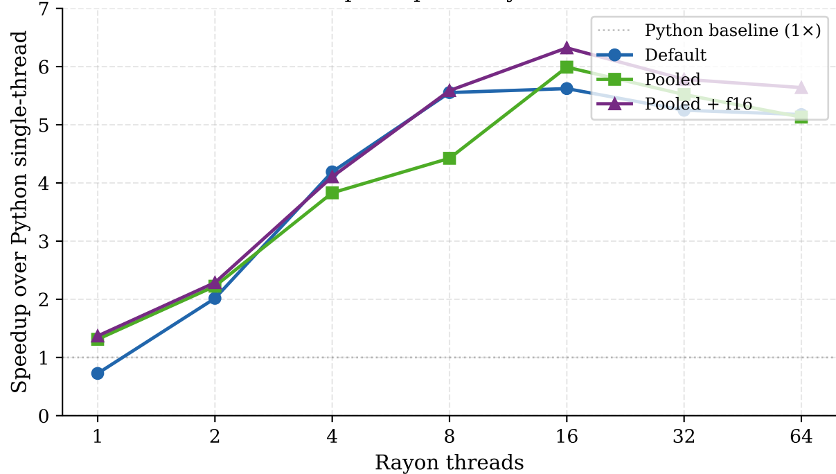
Speedup over Python
