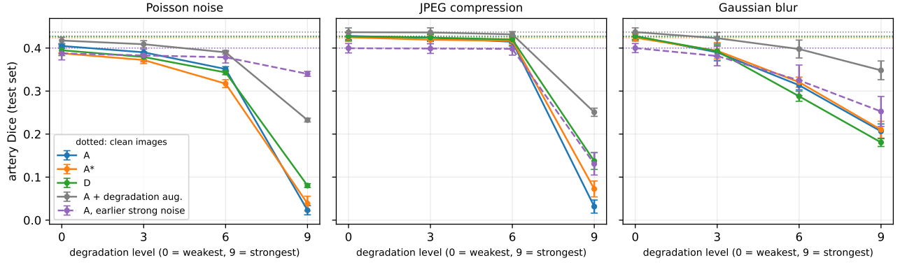
Fig. 15: Artery Dice on degraded test images (mean \pm standard deviation over three seeds; dotted lines: clean images). A, A* and D collapse under the strongest Poisson noise and JPEG compression; training A with realistic degradations restores a large part of the robustness that the overly strong noise augmentation of the earlier version (dashed) provided by accident.
