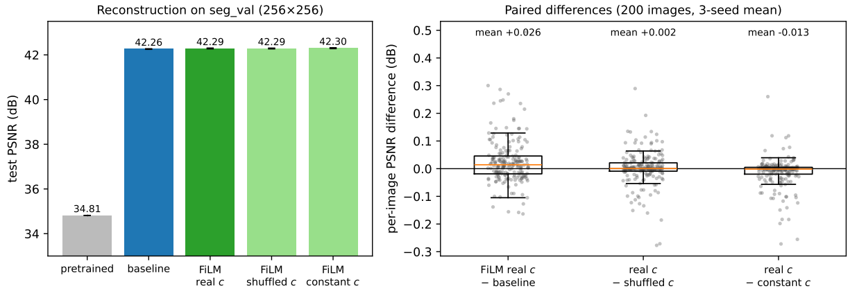
Fig. 7: Left: test PSNR per model (mean \pm standard deviation over 3 seeds). Right: per-image paired PSNR differences, averaged over the 3 seeds; the dots are the 200 test images.
