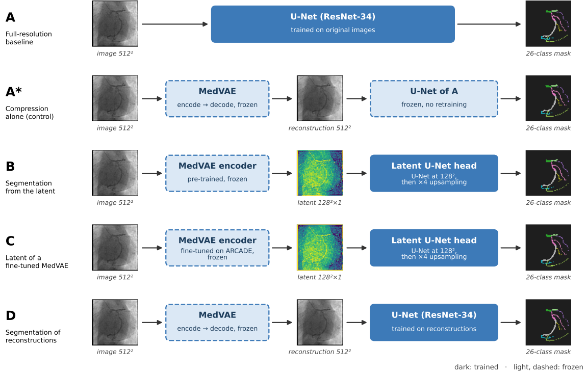
Fig. 12: The five segmentation conditions, illustrated on a test image: the input angiography, the MedVAE latent or reconstruction, and the 26-class mask. Dark boxes are trained, light dashed boxes are frozen. The trivial-compression controls R and A ↓ (not shown) replace MedVAE by a 4 \times 4 average pooling.
