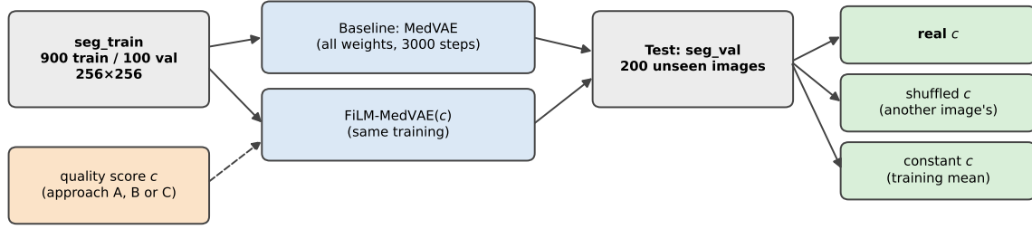
PSNR, vessel PSNR, SSIM, HaarPSI · 3 seeds · paired per-image differences If the model uses c : real c > shuffled c and real c > constant c
