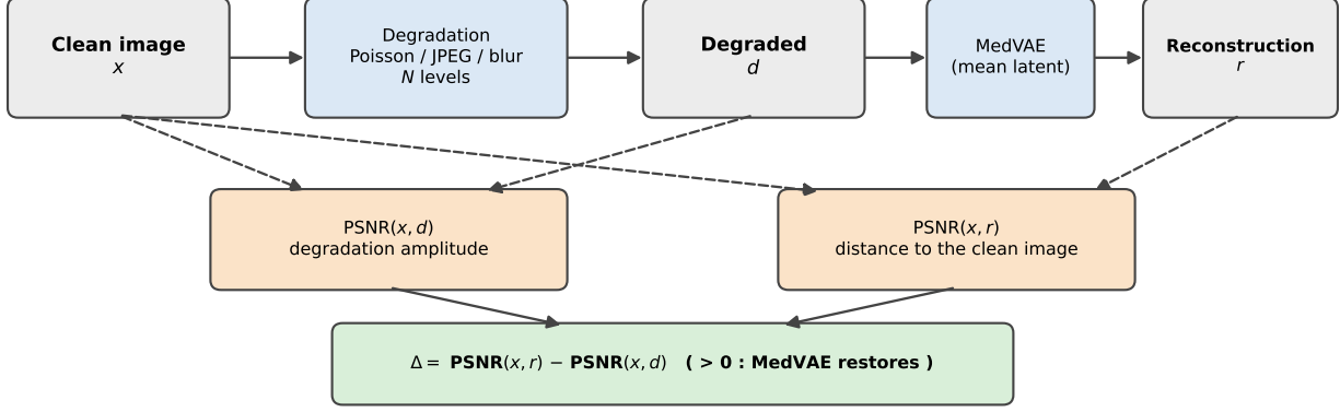
Fig. 1: Evaluation pipeline. A batch of clean images is degraded in a controlled manner over N levels, then reconstructed by MedVAE. The reconstruction is compared to the clean image, and the restoration gain \Delta (Eq. 1) compares this distance to that of the degraded input. A separate sweep is conducted per degradation type (Poisson, JPEG, blur).
