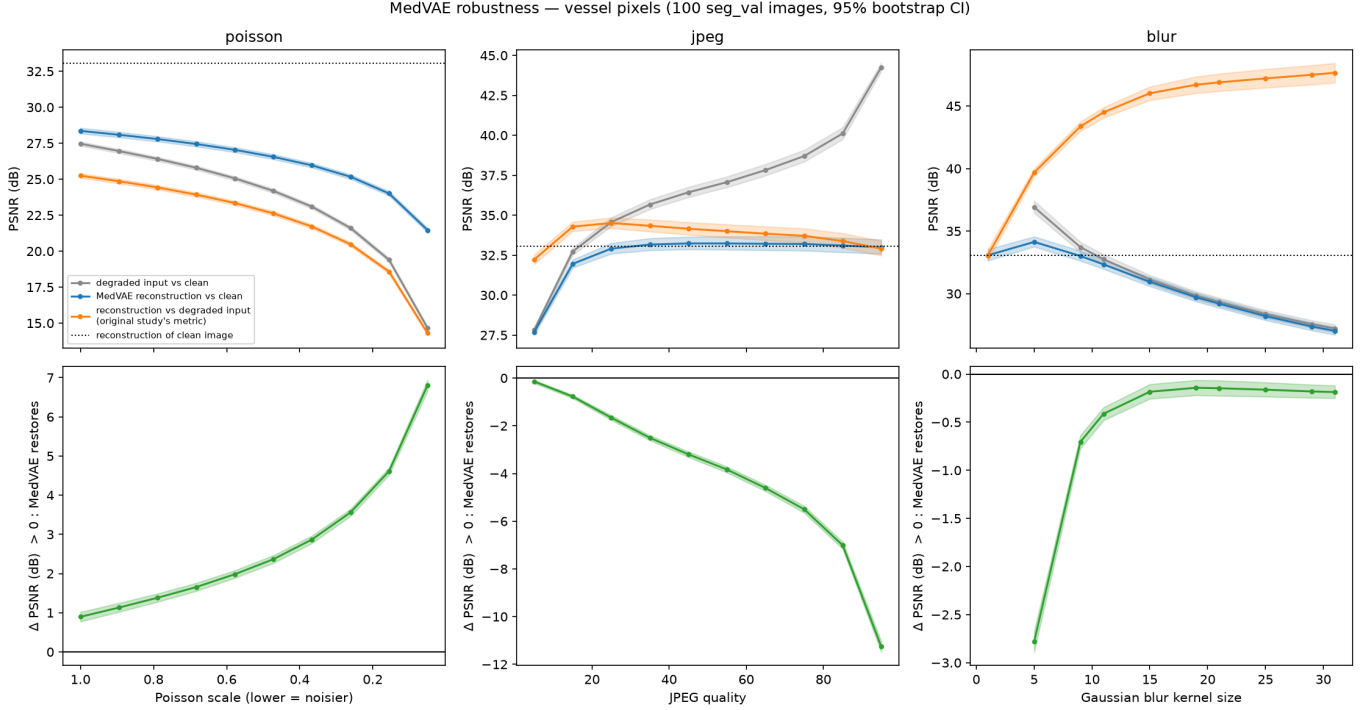
Fig. 2: Robustness of MedVAE on vessel pixels (100 seg_val images, 95% bootstrap confidence intervals). Top: PSNR of the degraded input (grey) and of MedVAE’s reconstruction (blue) with respect to the clean image; in orange, the fidelity of the reconstruction to the degraded input, the measure used in the earlier version of this study. Bottom: restoration gain \Delta ; positive values mean that MedVAE brings the image closer to the clean one.
