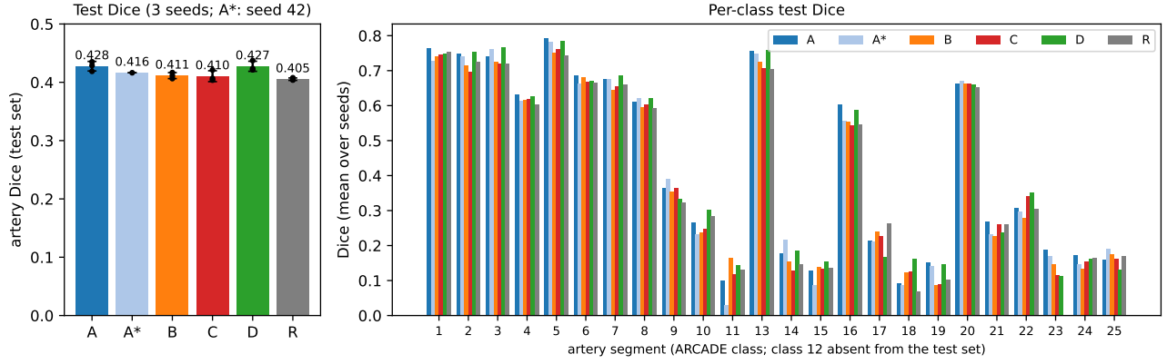
Fig. 13: Left: artery Dice on the test set per condition (bars: mean over seeds, dots: individual seeds). Right: per-class Dice, averaged over seeds. Conditions A, A* and D are nearly indistinguishable; B and C follow the same per-class profile a few points lower, with the largest gaps on thin, rare segments, and the trivial-compression control R is close to them. A*: seed-42 model.
