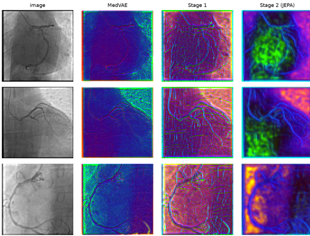
Fig. 11: RGB PCA of the encoder features before conv_out for three test angiographies (PCA fitted on 50 other test images; pre-training seed 42). Columns: image, MedVAE, stage 1, stage 2.
