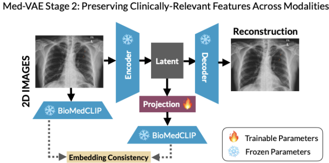
Fig. 8: Original stage 2: latent space alignment on BioMedCLIP embeddings.
