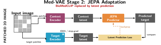
Fig. 9: Modified stage 2: JEPA adaptation — the context encoder predicts the target latent of the EMA encoder (stop-grad).
