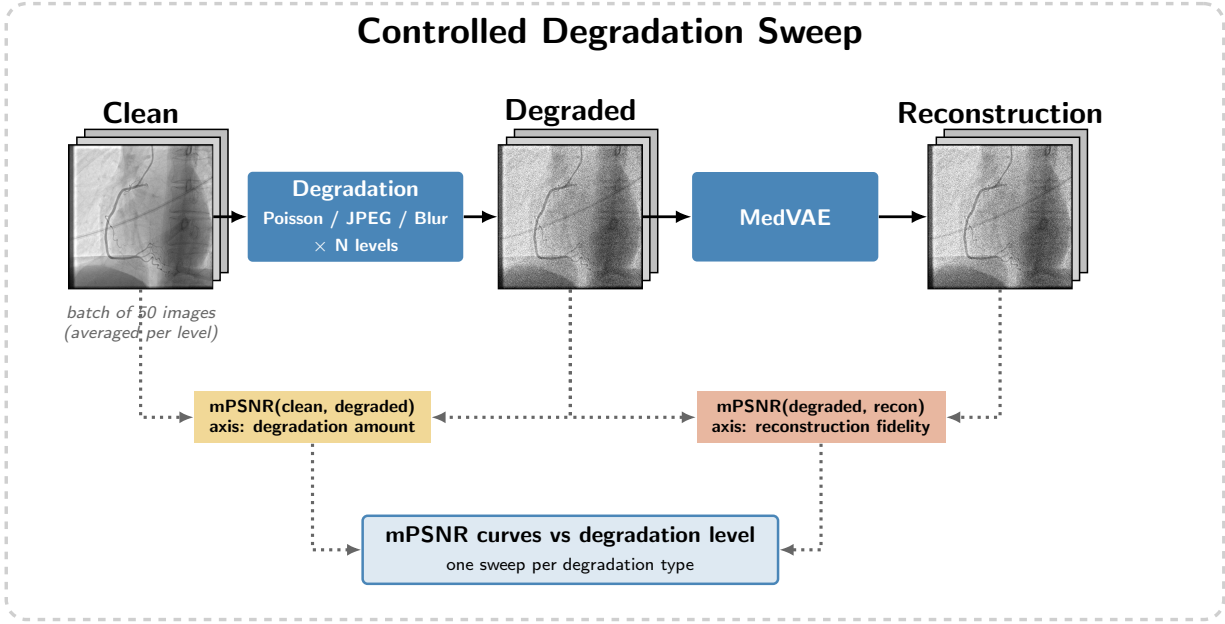
Fig. 1: Evaluation pipeline. A batch of clean images is degraded in a controlled manner over N levels, then reconstructed by MedVAE. Two vessel-masked measures are computed per level and averaged over the batch: mPSNR(clean, degraded) quantifies the amplitude of the applied degradation, and mPSNR(degraded, recon) the reconstruction fidelity. A separate sweep is conducted per degradation type (Poisson, JPEG, blur).
