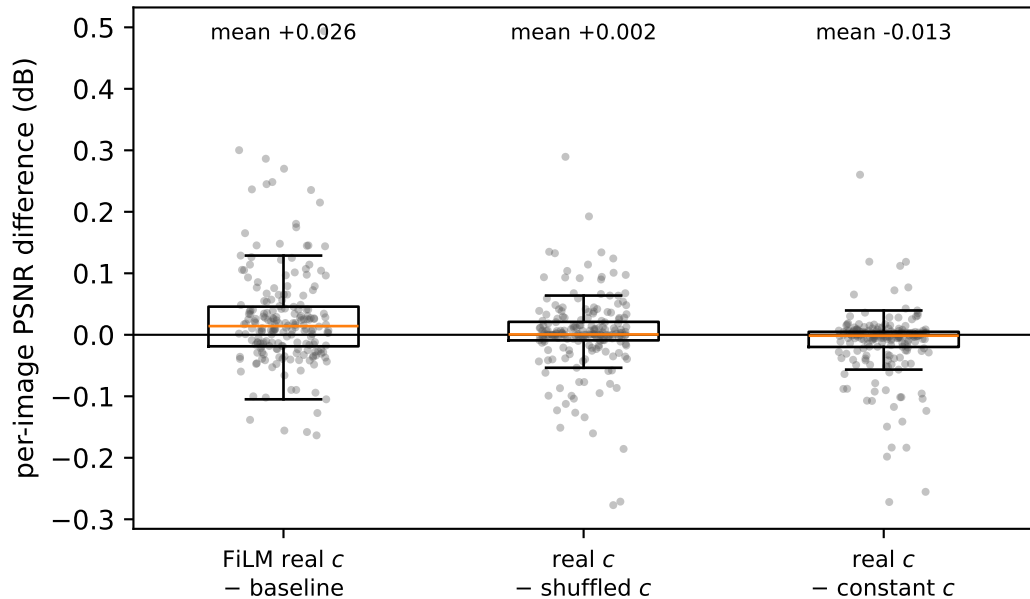
Paired differences (200 images, 3-seed mean)
