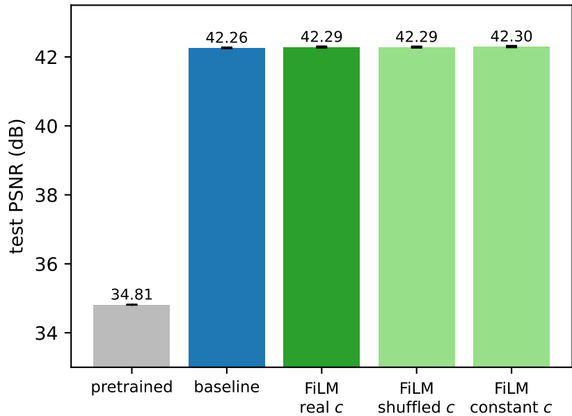
Reconstruction on seg_val (256×256)
