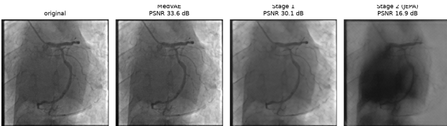
Fig. 10: Reconstruction of a test image by MedVAE, stage 1 and stage 2 (left to right after the original).
