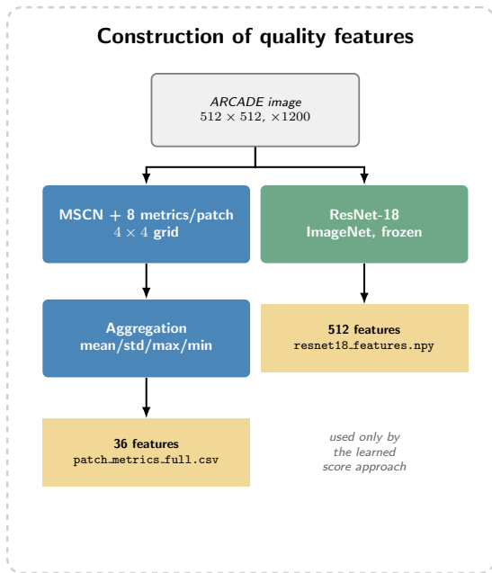
Fig. 3: Construction of quality features: per-patch IQA metrics and ResNet-18 features.
