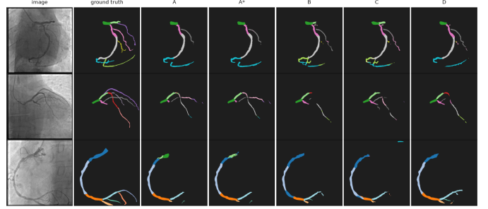
Fig. 16: Predictions of the seed-42 models on three test images (one colour per artery segment). A, A* and D are nearly identical; B and C, which segment from the 128 \times 128 latent, recover the main tree with slightly less regular contours and miss or confuse some thin branches.
