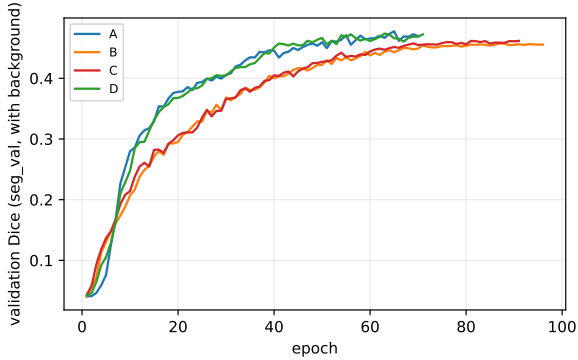
Fig. 14: Validation Dice during training (mean over the three seeds). B and C, which segment from the compressed latent, learn more slowly and plateau a few points below A and D.
