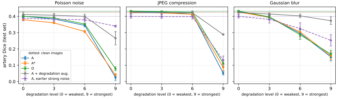
Fig. 15: Artery Dice on degraded test images (mean \pm standard deviation over three seeds; dotted lines: clean images). A, A* and D collapse under strong degradations; training A with realistic degradations restores most of the robustness that the overly strong noise augmentation of the earlier version (dashed) provided by accident.
