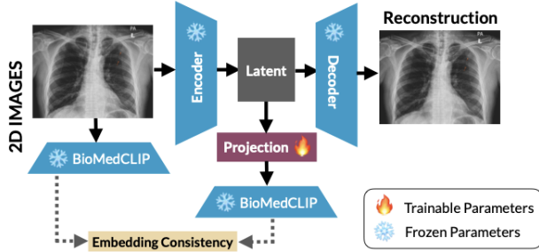
Fig. 8: Original stage 2: latent space alignment on BioMedCLIP embeddings. Reproduced from Varma et al. [1], Fig. 1b.
