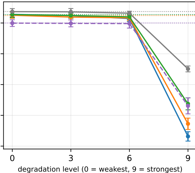
JPEG compression
