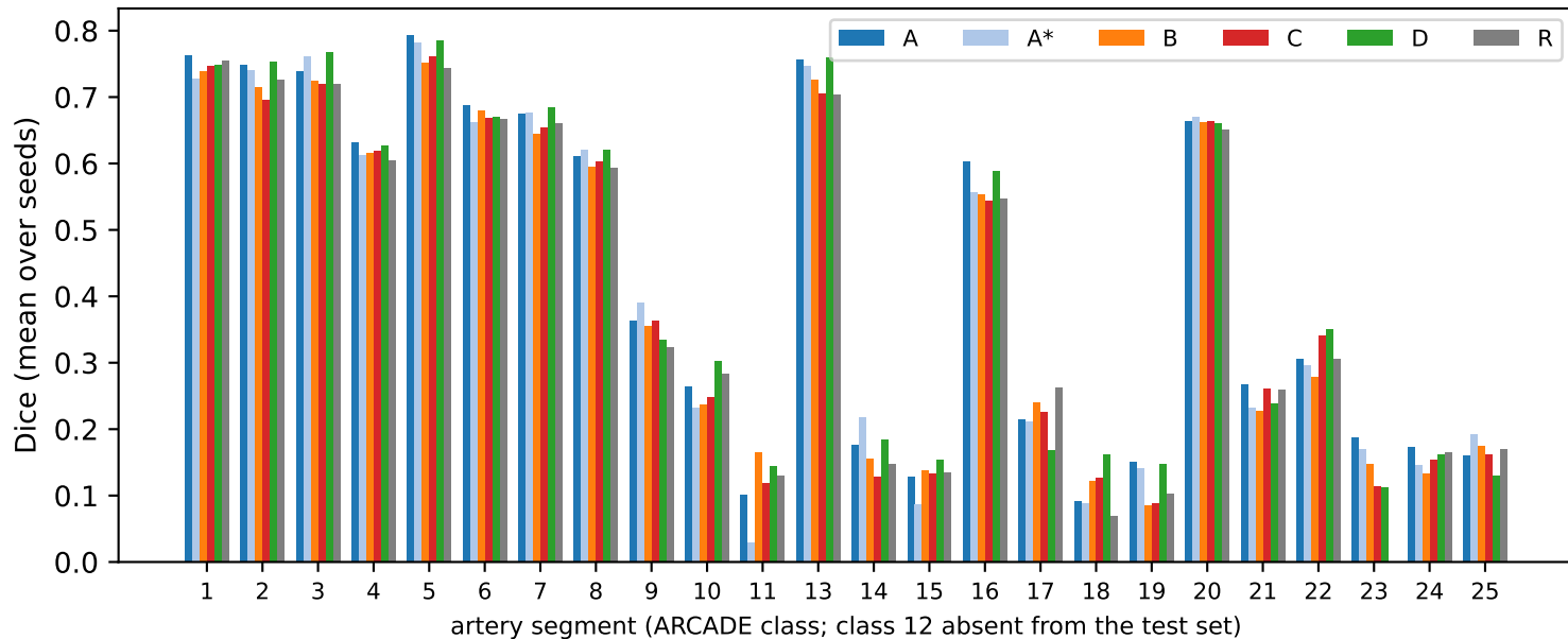
Per-class test Dice
