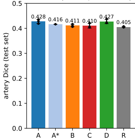
Test Dice (3 seeds; A*: seed 42)
