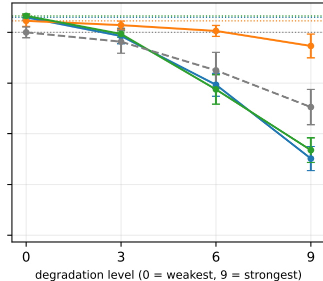
Gaussian blur
