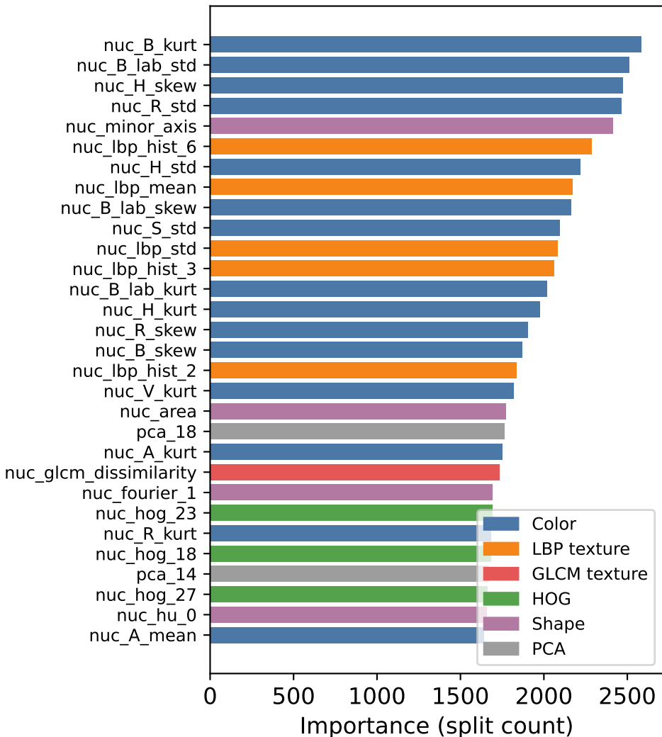
Top-30 features (LightGBM split counts)
