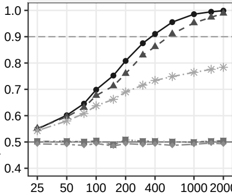
Set 3, combined (mean and SD matched)
