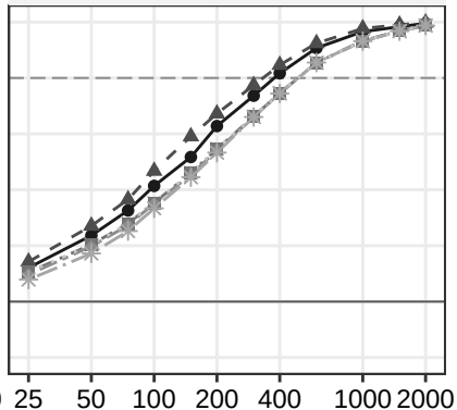
Set 4, location shift of everyone (control: KS's home turf)
