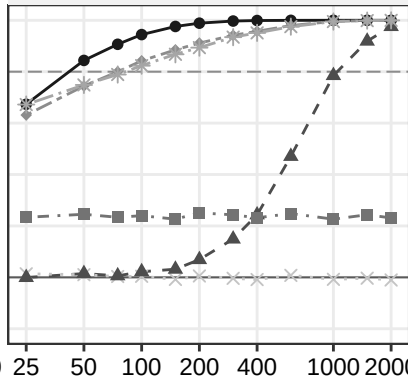
Set 4, extremes further out (mean matched)
