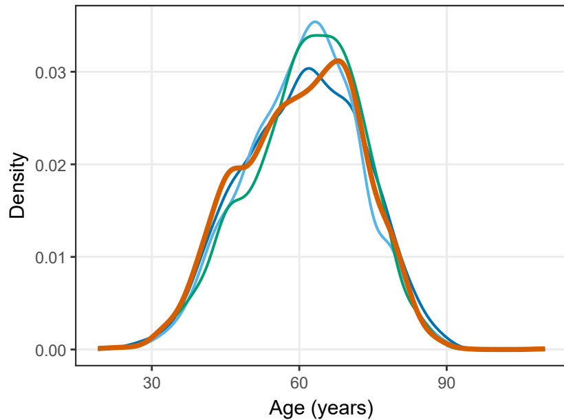
(a) Age
