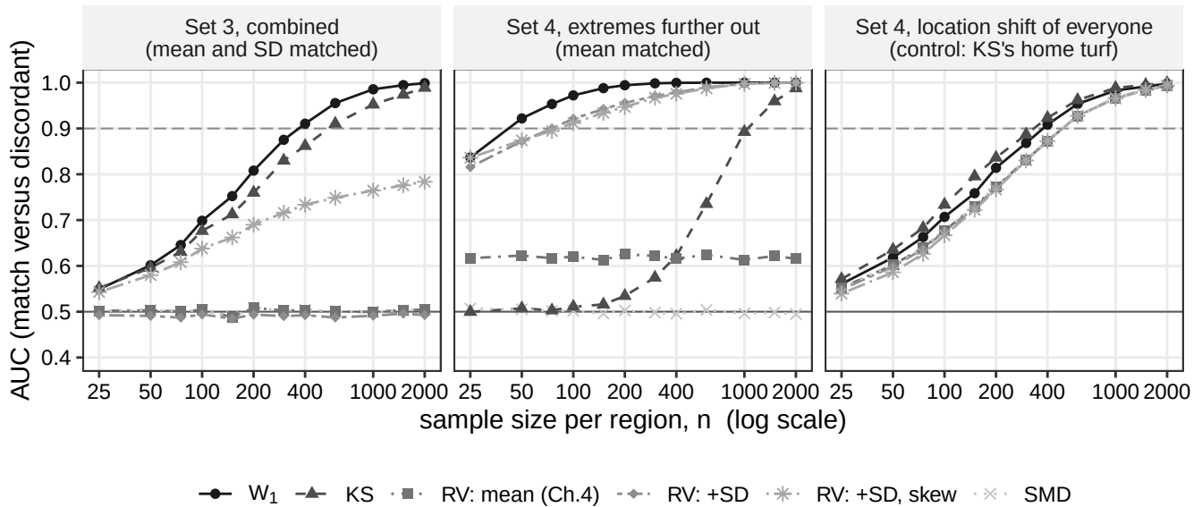
FIGURE 2 Selection AUC (true matches versus discordant candidates) as a function of per-region sample size ( n = 25 –2,000, log scale) for six distance measures in three cells of Study 1: the Set 3 combined cell (mean- and SD-matched mixtures), the Set 4 symmetric-severity cell (mean-matched displaced extremes), and the Set 4 bulk-shift control cell (uniform location shift of the whole population). The dashed horizontal line marks AUC = 0.9; chance corresponds to 0.5.
